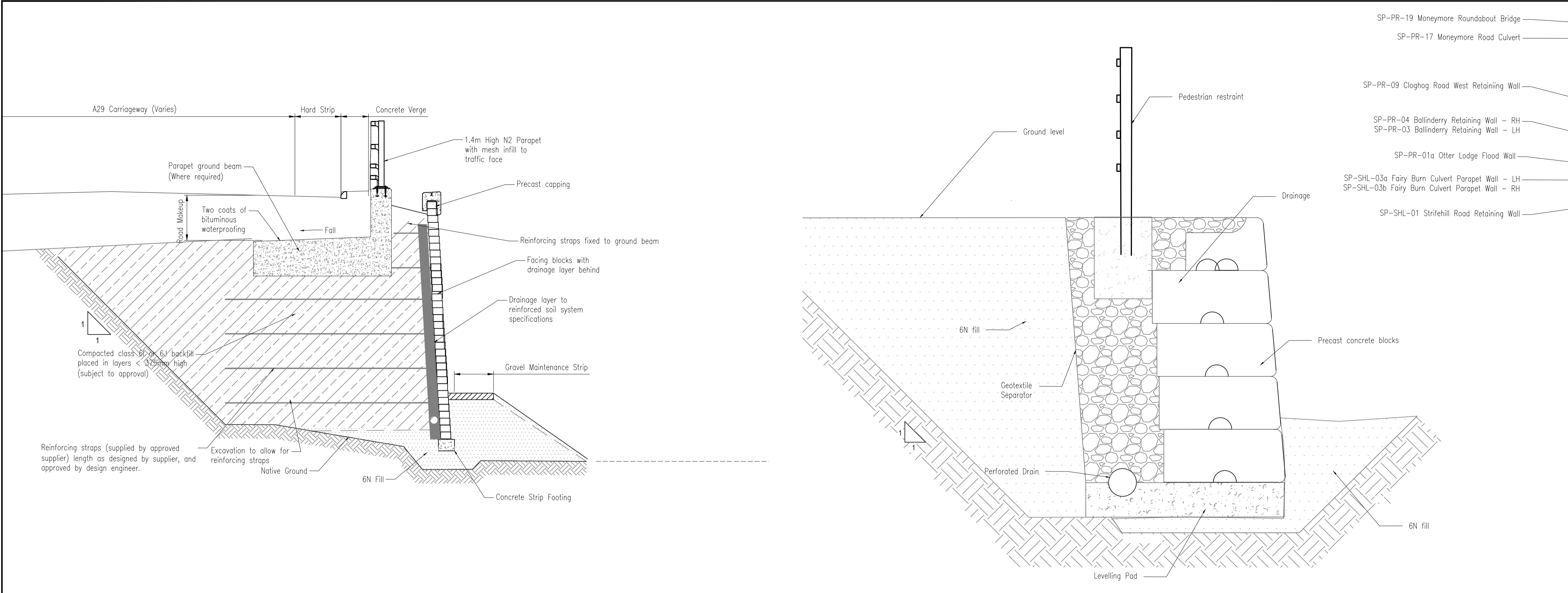
BLOCK GRAVITY WALL CROSS SECTION Scale 1:20
