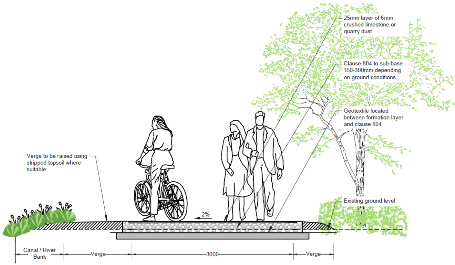
TYPICAL UNBOUND SURFACE SCALE 1:25
