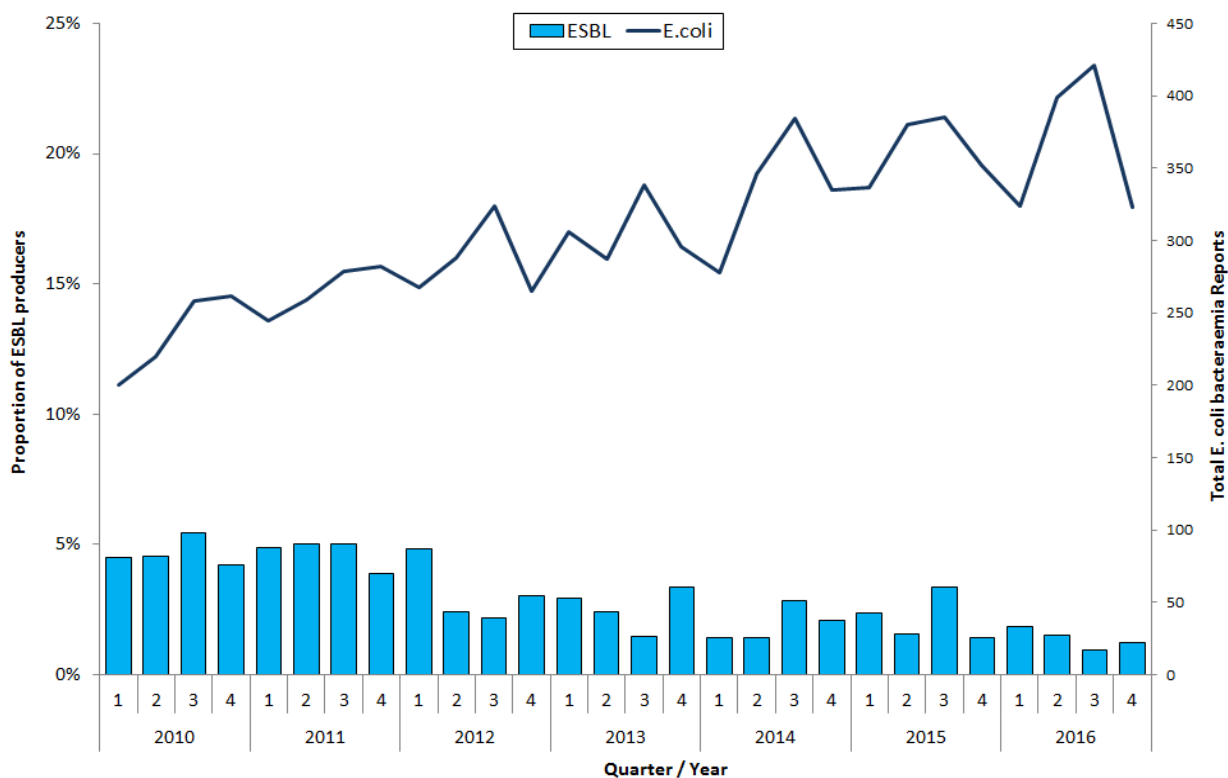
Fig 2: Total E.coli and proportion of ESBL producers in NI, by quarter, from 2010 to 2016 (Q4)
