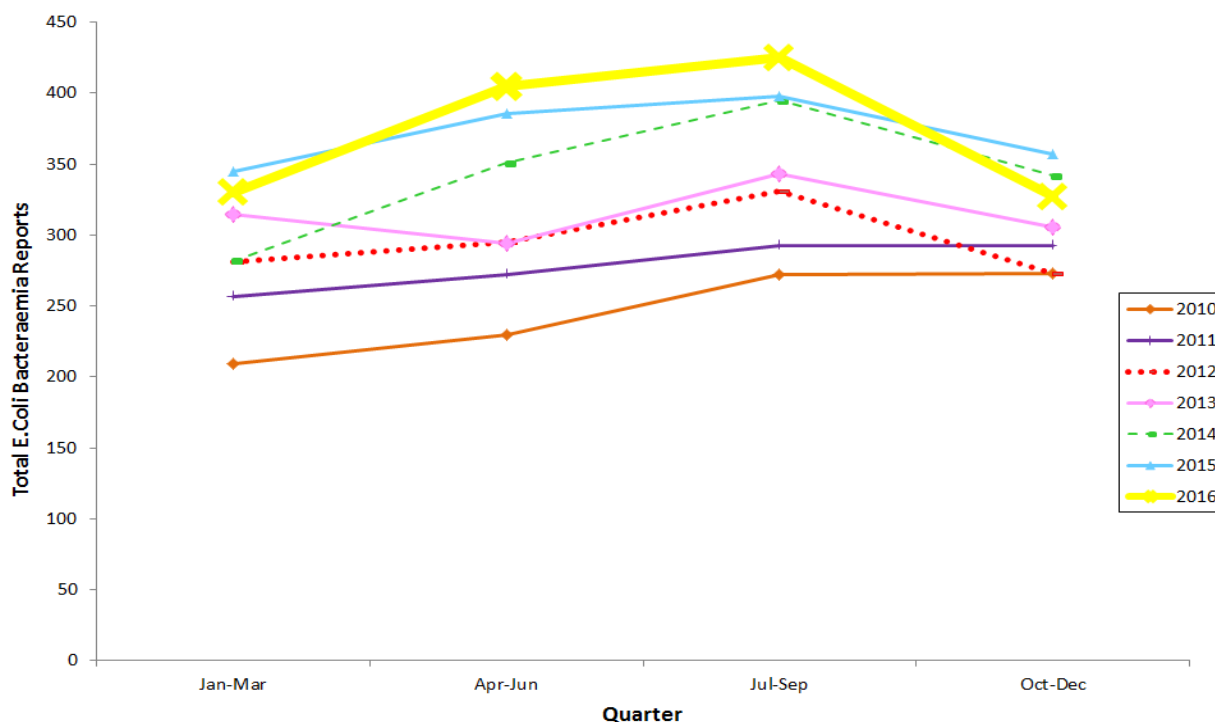
Fig 1: Total E.coli bacteraemias in NI, by quarter, from 2010 to 2016 (Q4)
