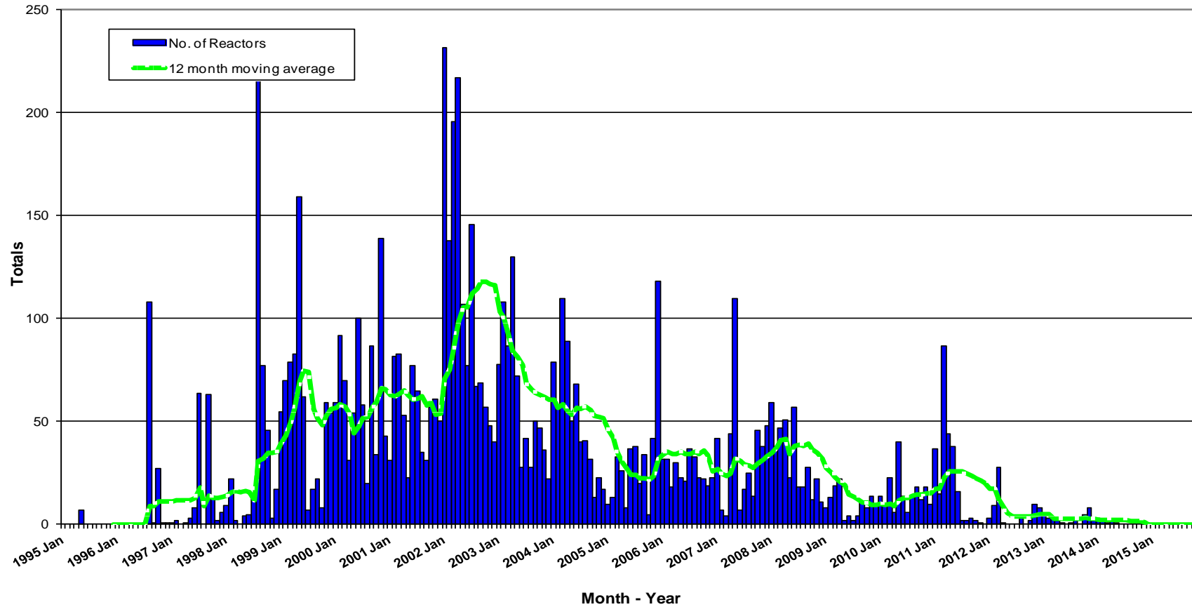
BR Reactors: January 1995 to November 2015
