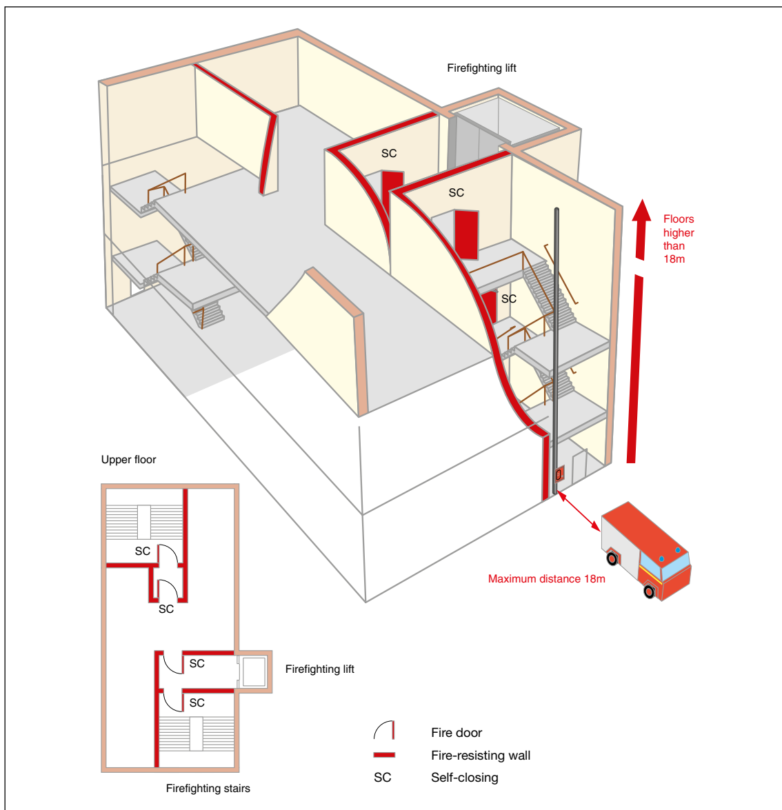
Figure 55: Tall building with a firefighting shaft
