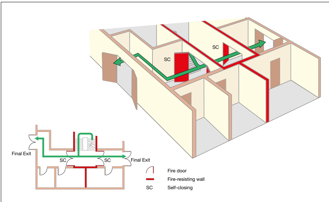
Figure 43: Example of two escape routes from a stairway to final exits
