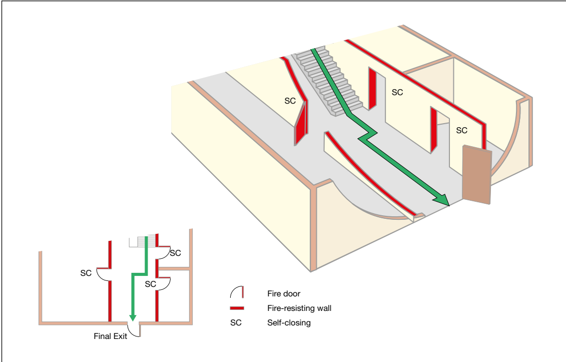
Figure 42: Example of a protected route from a stairway to a final exit
