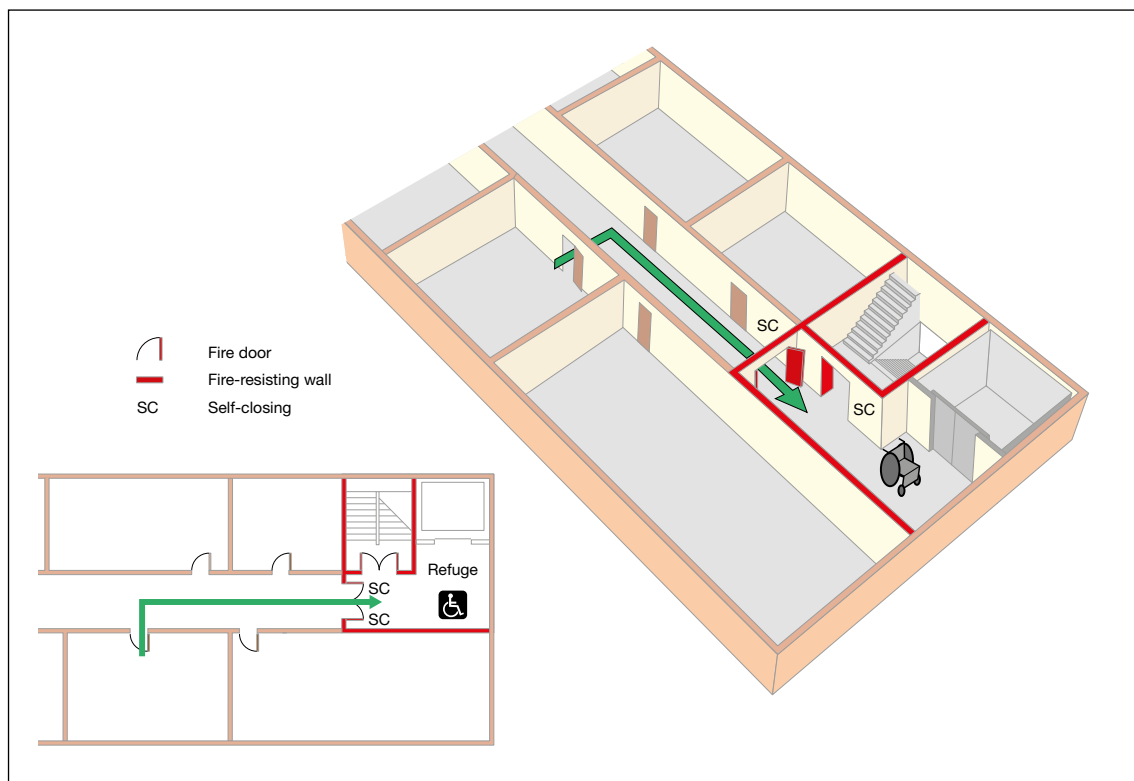
Figure 31: An example of a refuge
