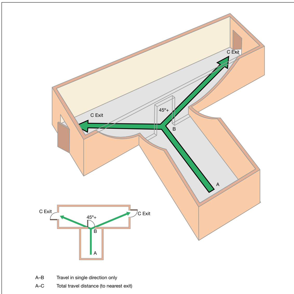
Figure 35: Measuring travel distance from initial dead end (inner room)
