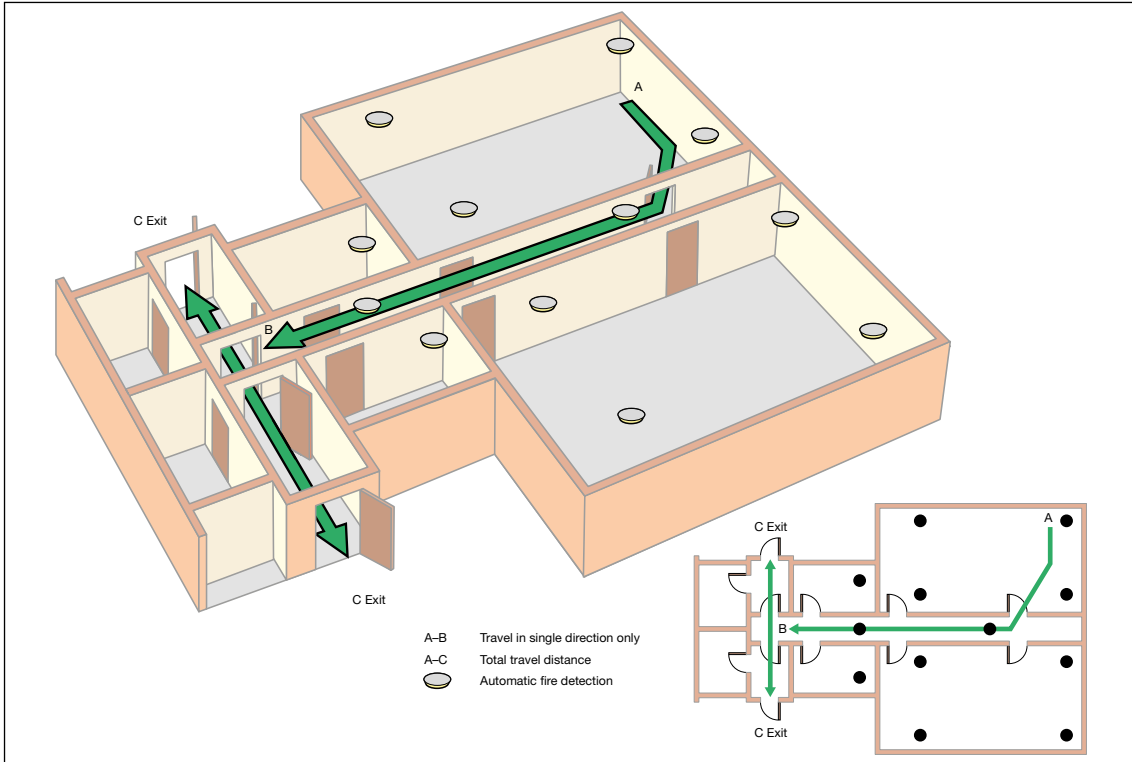
Figure 36: Dead-end condition with automatic fire detection
