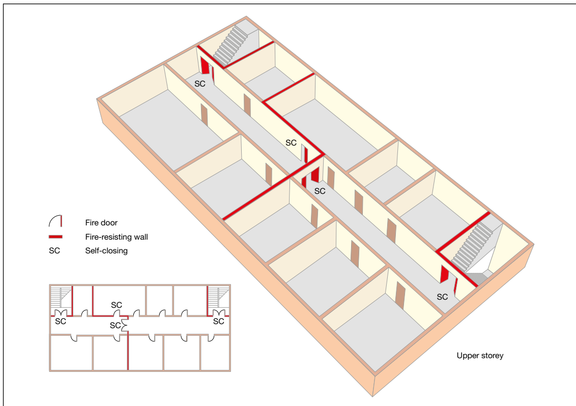
Figure 40: Subdivision of corridor between two stairways or exits
