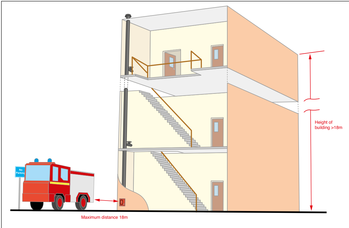
Figure 27: Rising main
