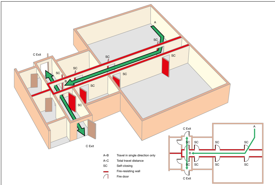
Figure 37: Dead-end condition with fire-resisting construction
