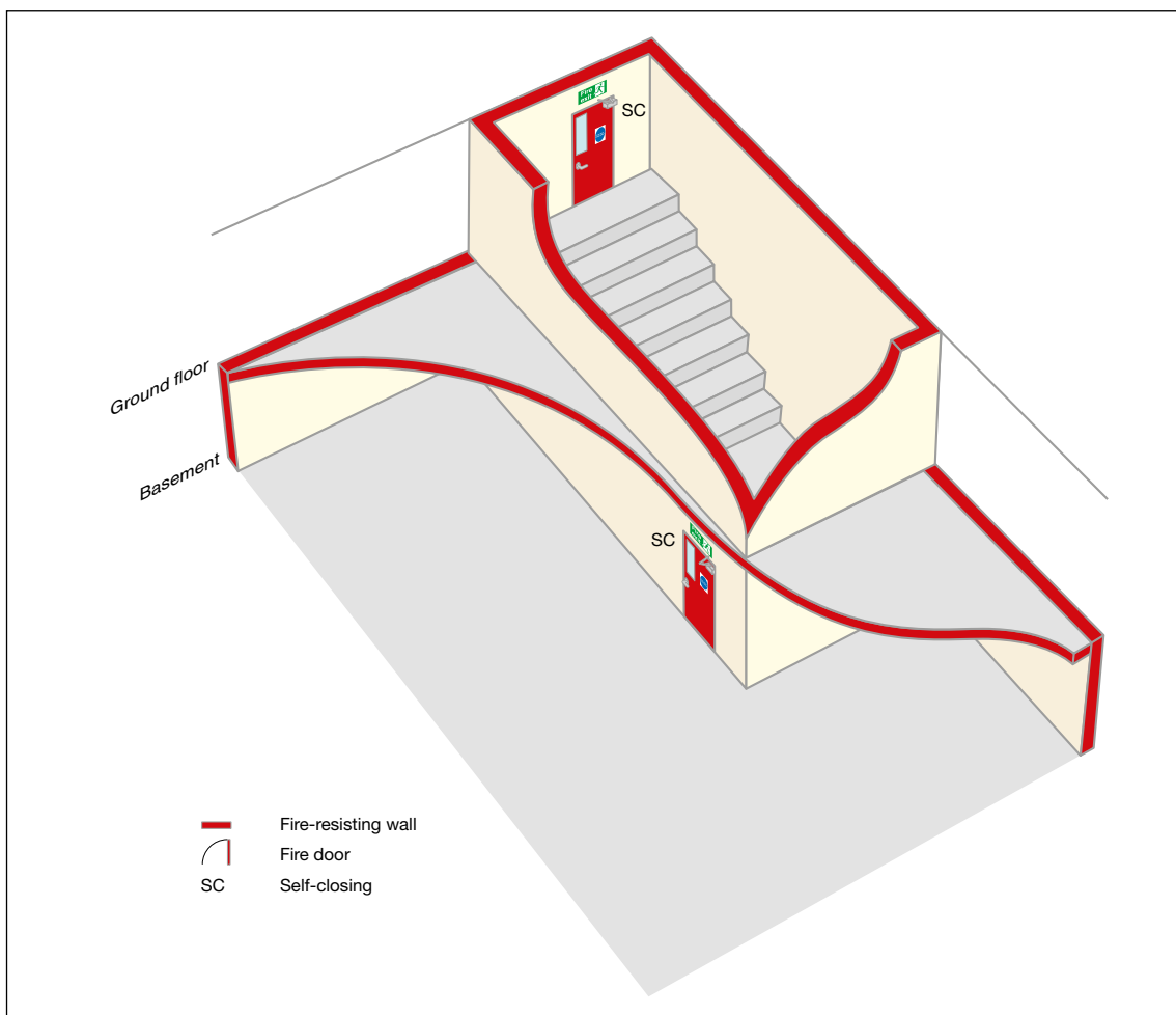
Figure 39: Basement protection
