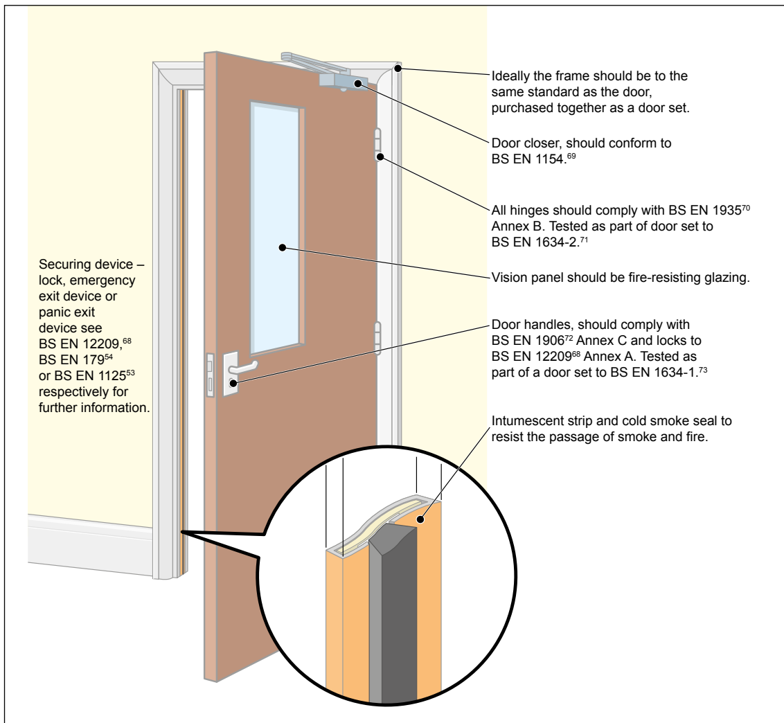
Figure 73: A fire-resisting and smoke stopping door
