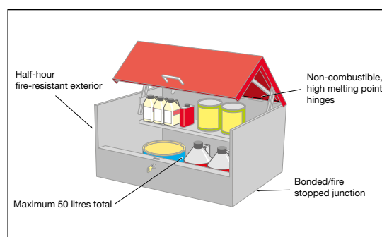
Figure 22: A 50 litre storage bin for flammables
