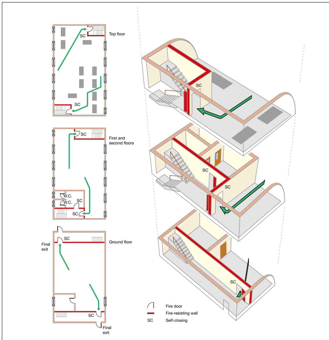
Figure 54: Four-storey premises: ground and up to three upper floors
