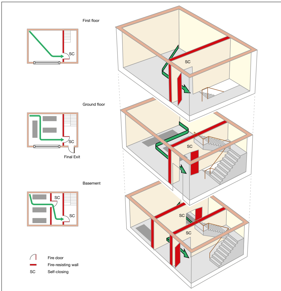
Figure 59: Three-storey premises: basement, ground and one upper floor
