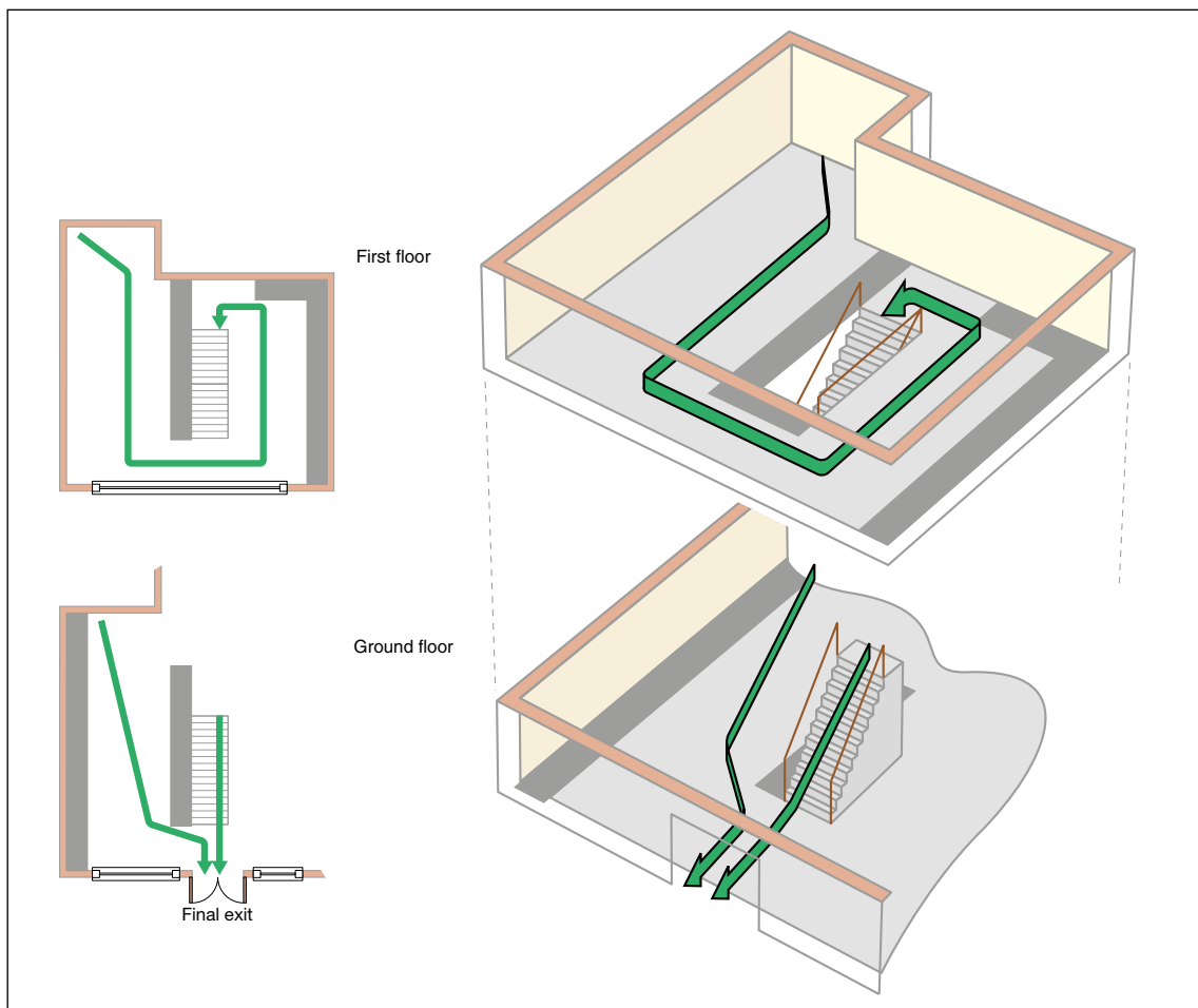
Figure 56: Two-storey premises: ground and one upper floor
