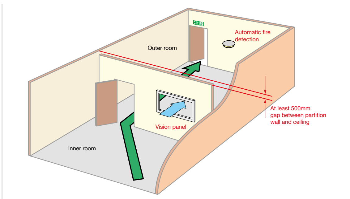
Figure 34: Inner rooms
