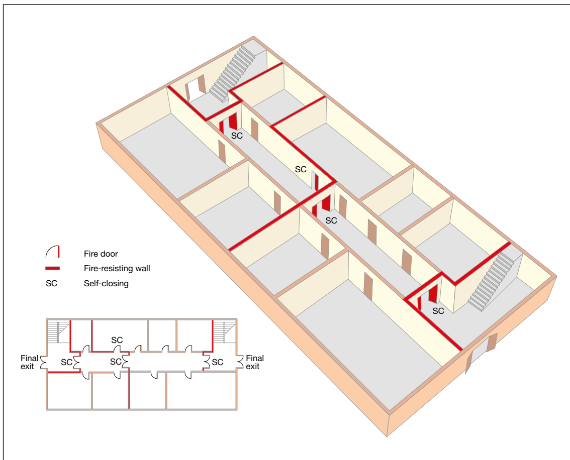
Figure 44: Separation of protected stairways
