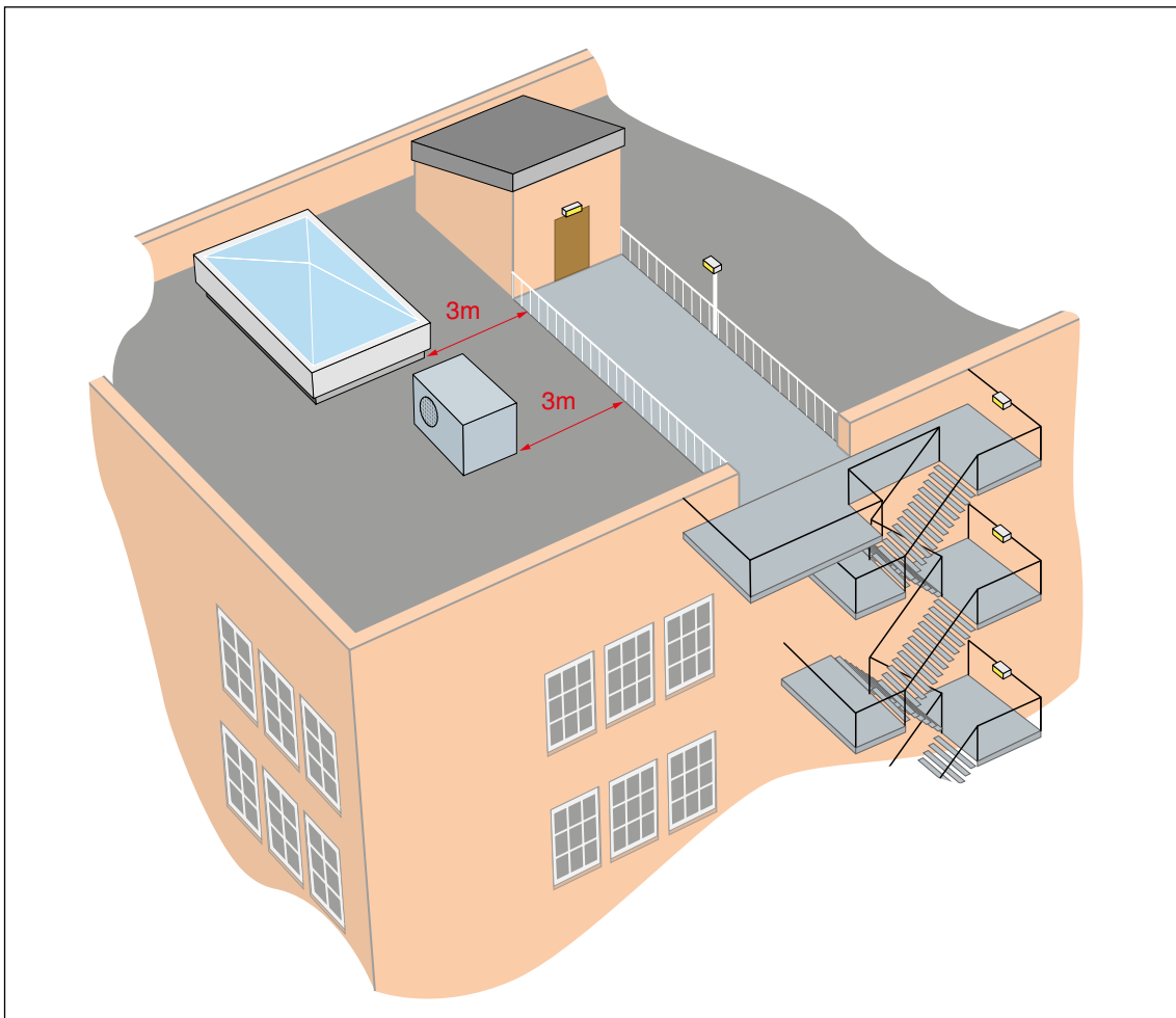
Figure 47: An escape route across a roof
