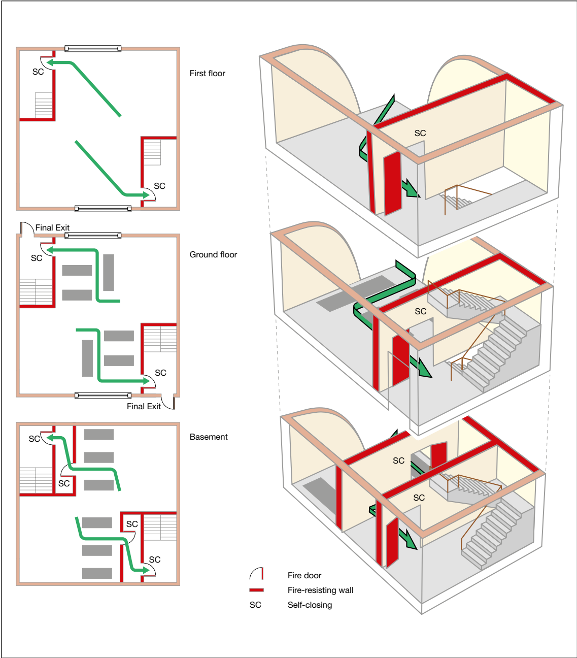
Figure 53: Three-storey premises: basement, ground and one upper floor
