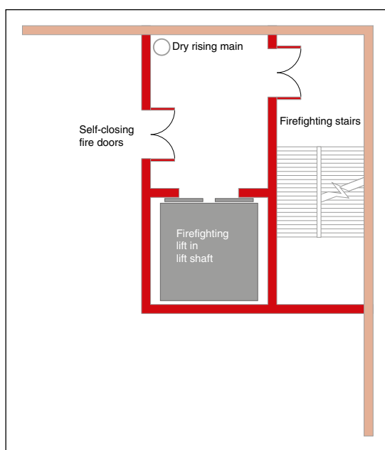
Figure 26: Firefighting shaft
