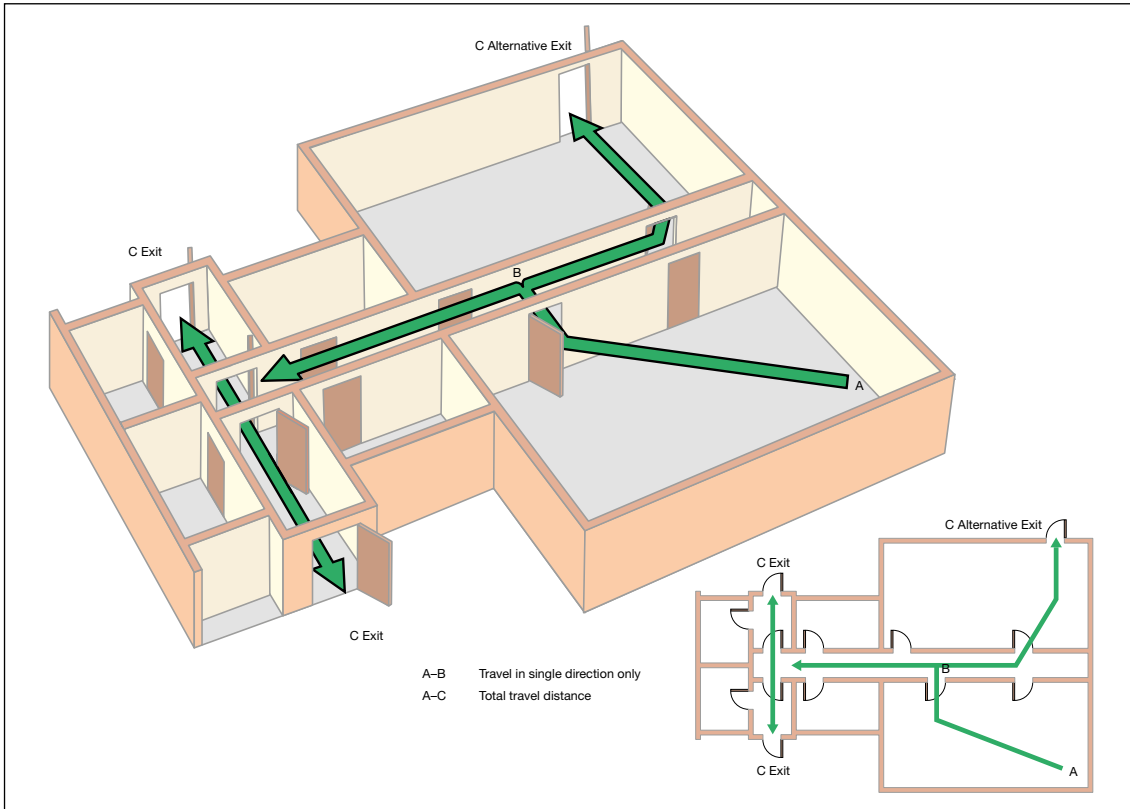
Figure 38: Dead-end condition provided with an alternative exit
