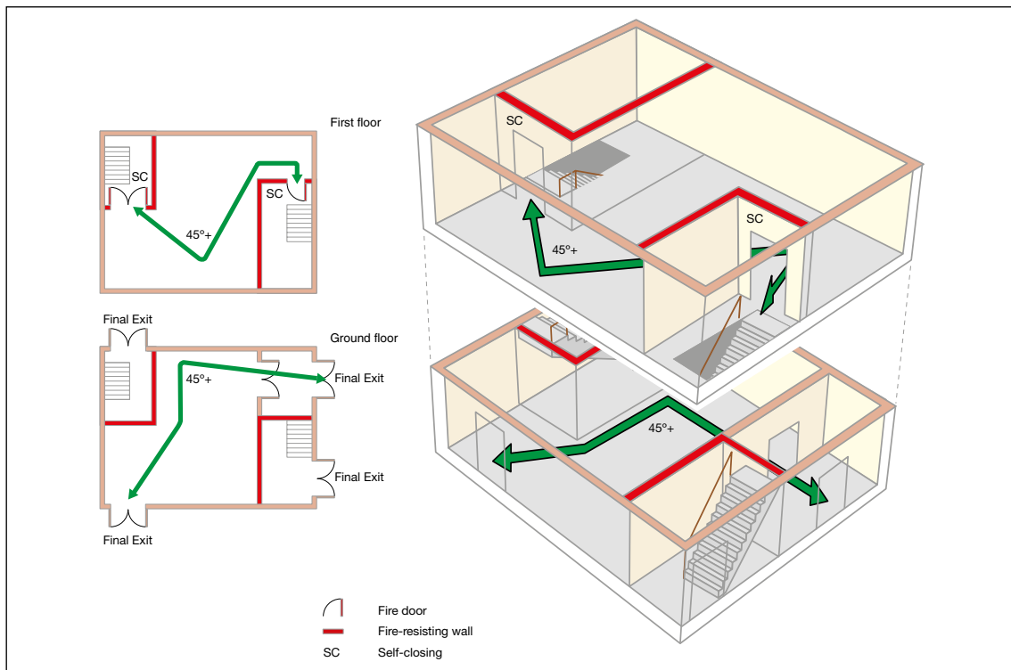
Figure 52: Two-storey premises: higher risk premises
