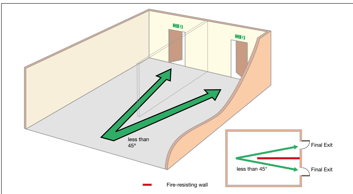
Figure 33: Alternative exits (separated by fire-resisting construction)
