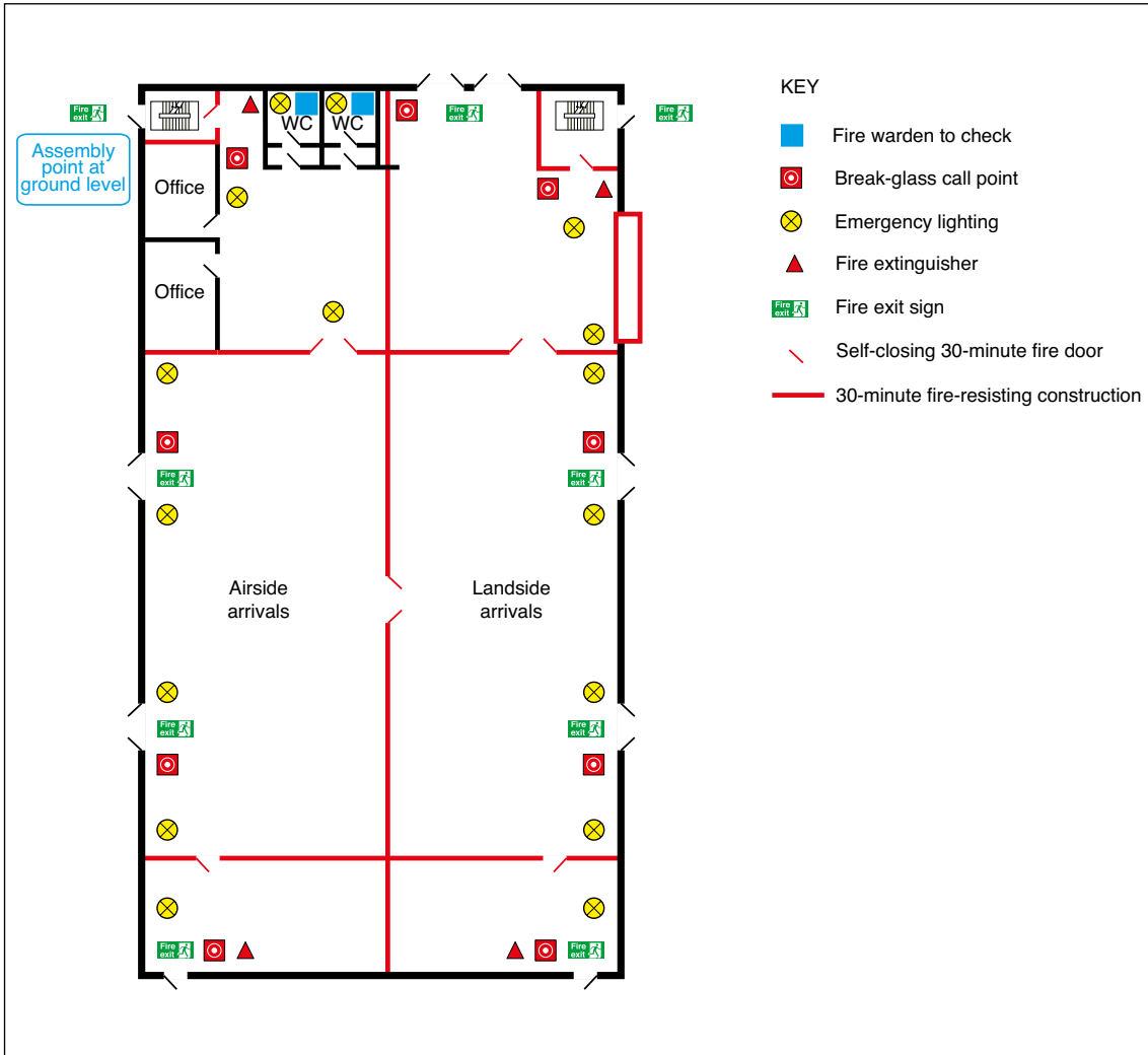
Figure 17: Example of a line drawing showing general fire safety precautions
