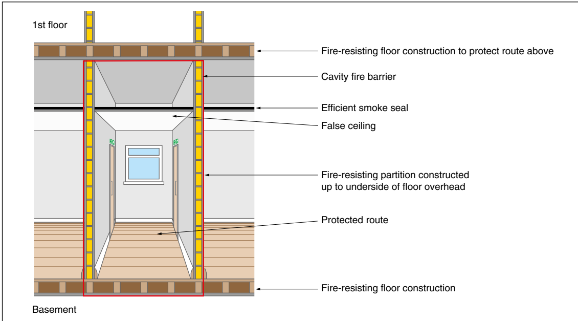
Figure 72: Fire-resisting construction
