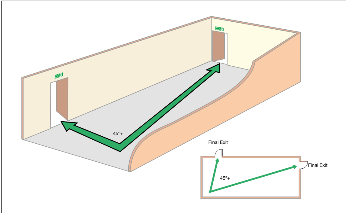
Figure 32: Alternative exits
