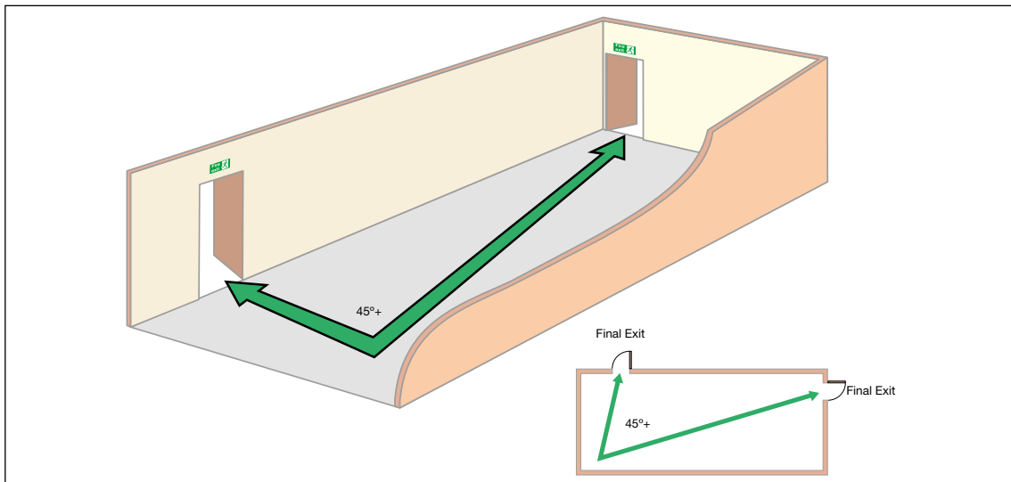
Figure 48: Ground floor premises with more than one exit
