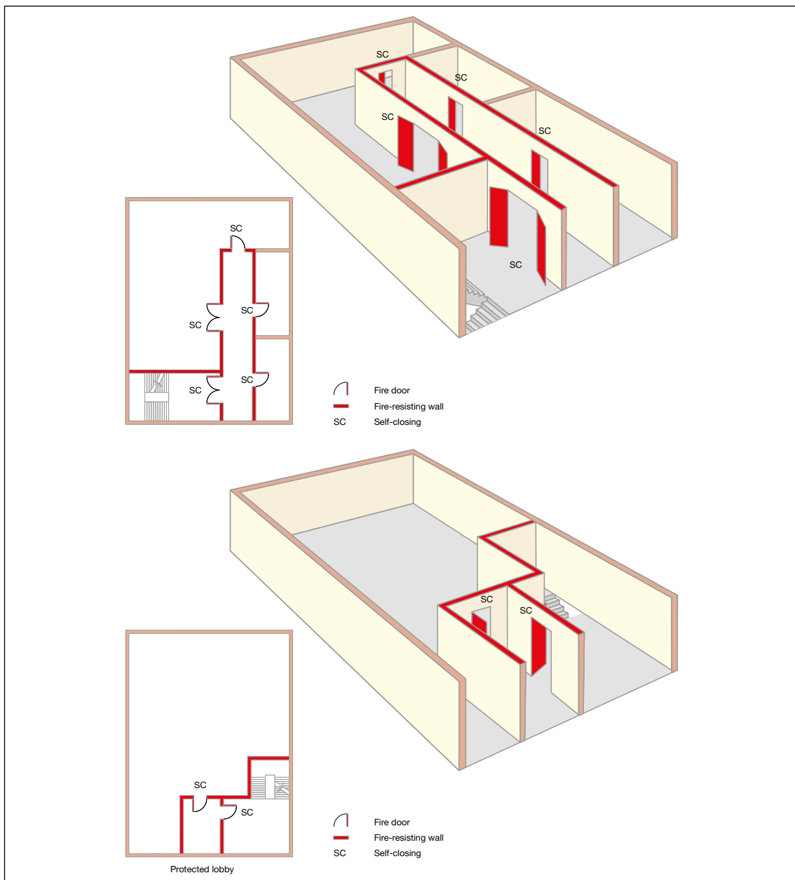
Figure 41: Examples of a Stairway with protected lobby/corridor approach
