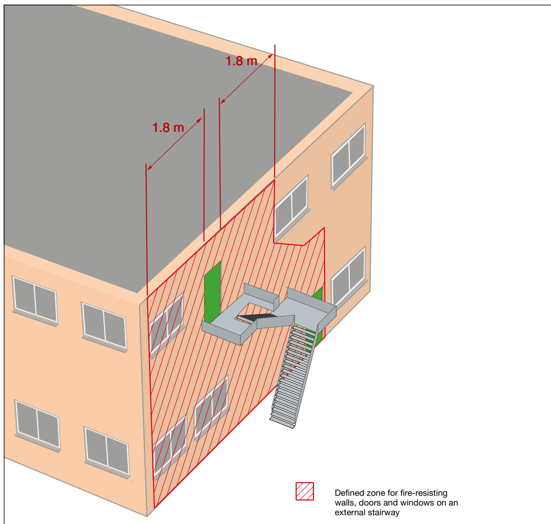
Figure 46: Protection to an external stairway
