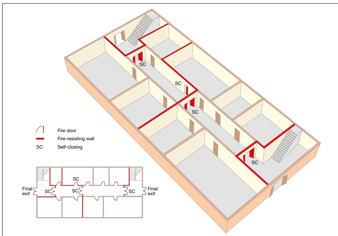
Figure 38: Separation of protected stairways
