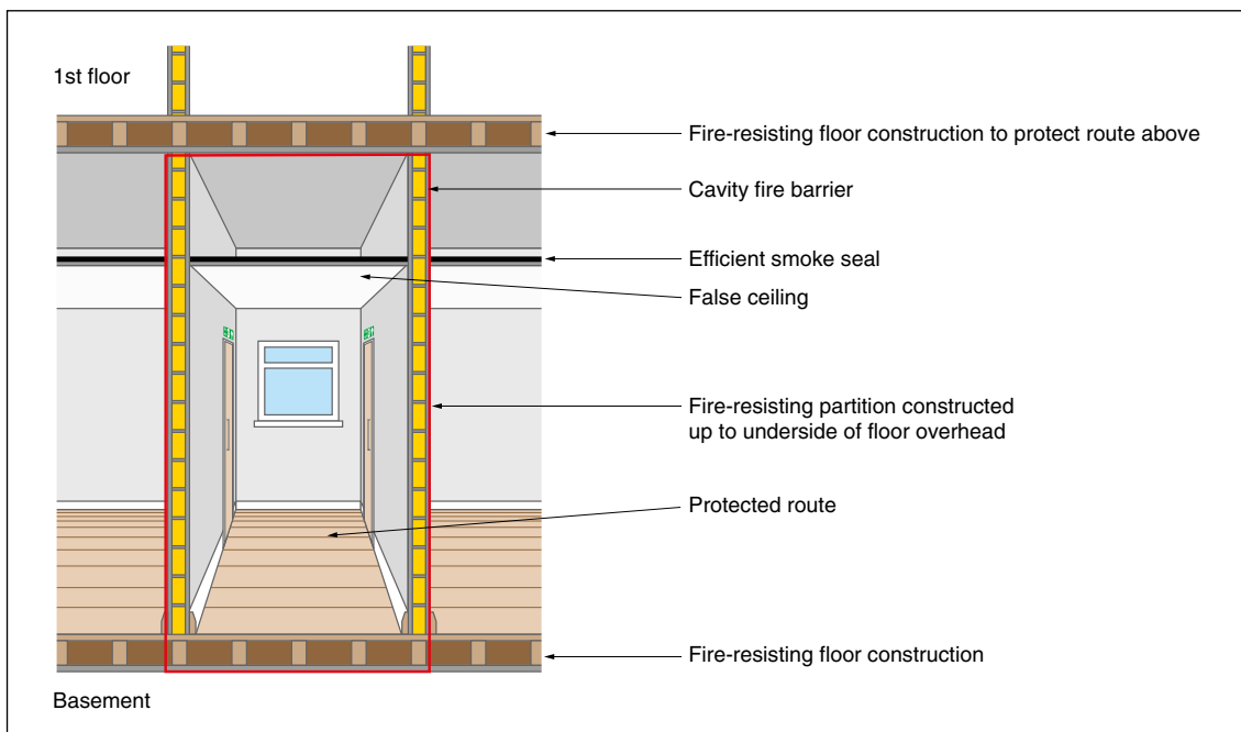
Figure 64: Fire-resisting construction
