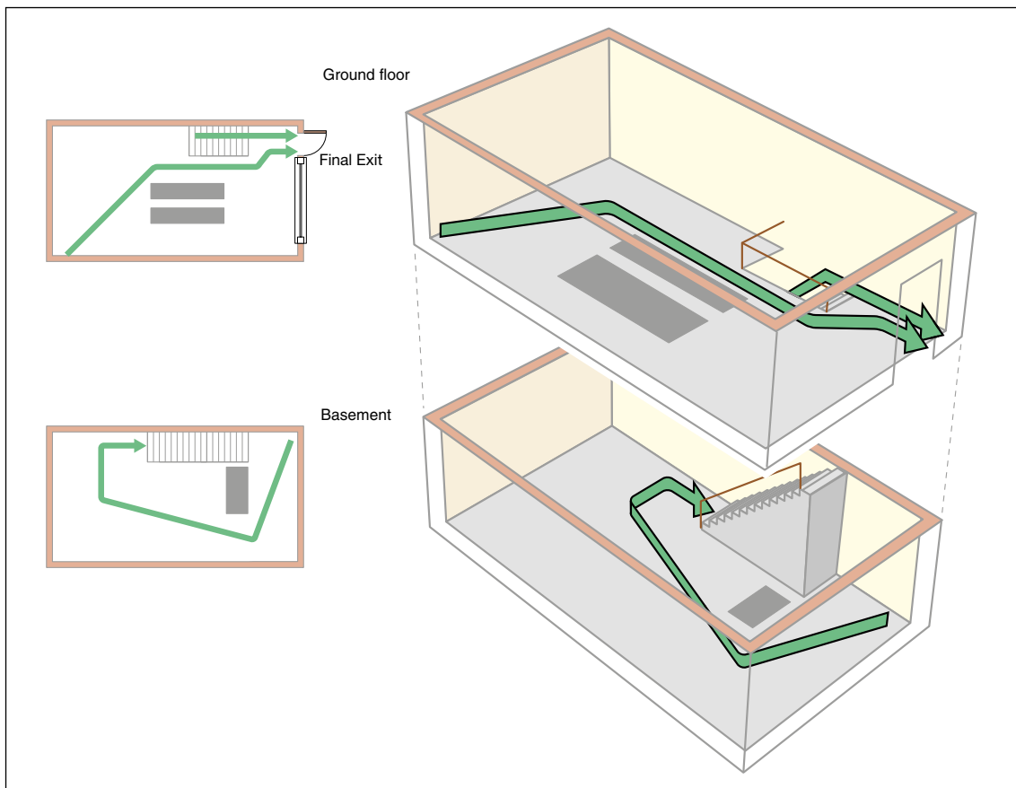
Figure 51: Two-storey premises, basement and ground floor
