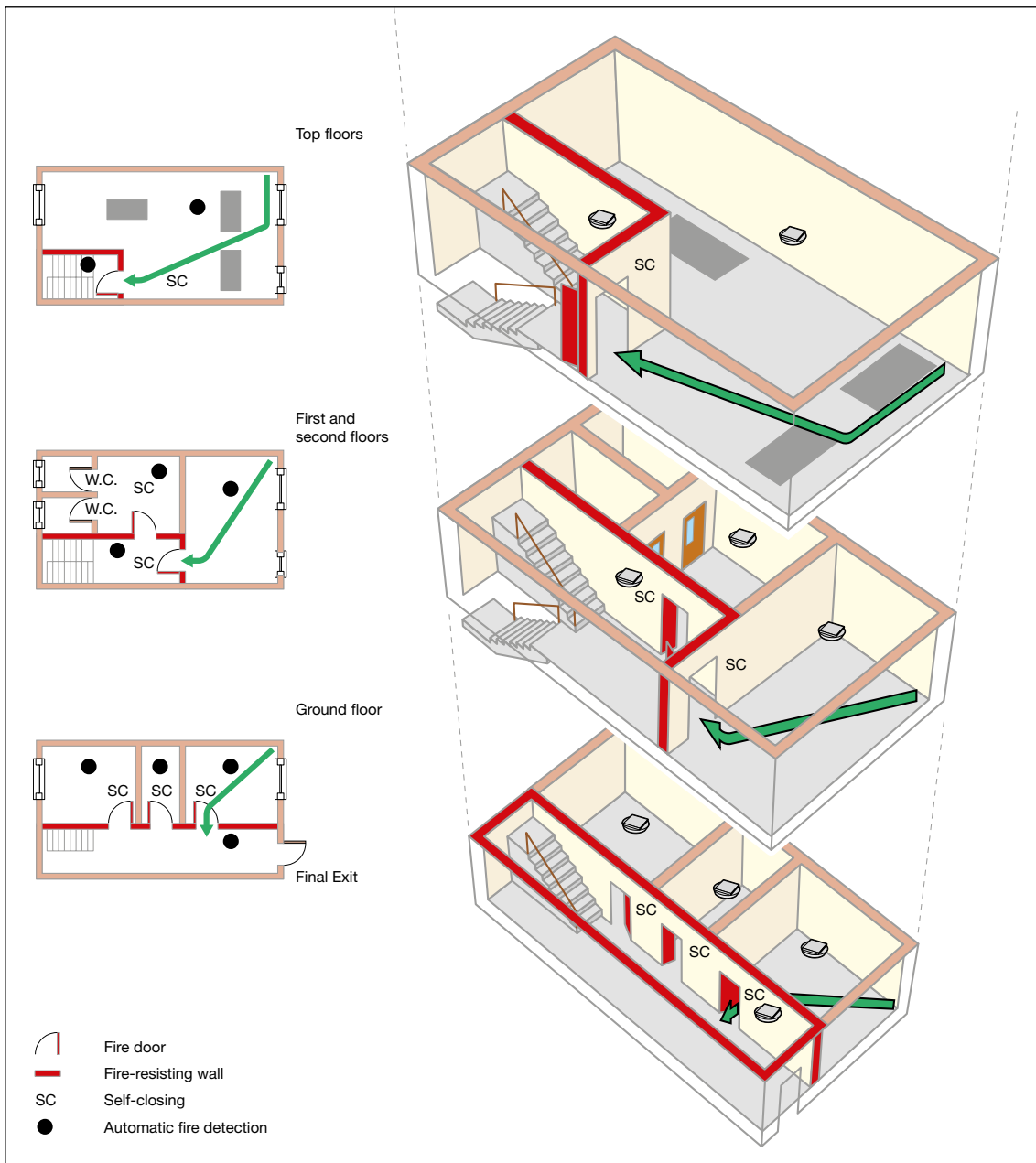
Figure 55: Four-storey, ground and up to three upper floors – protected with automatic fire detection
