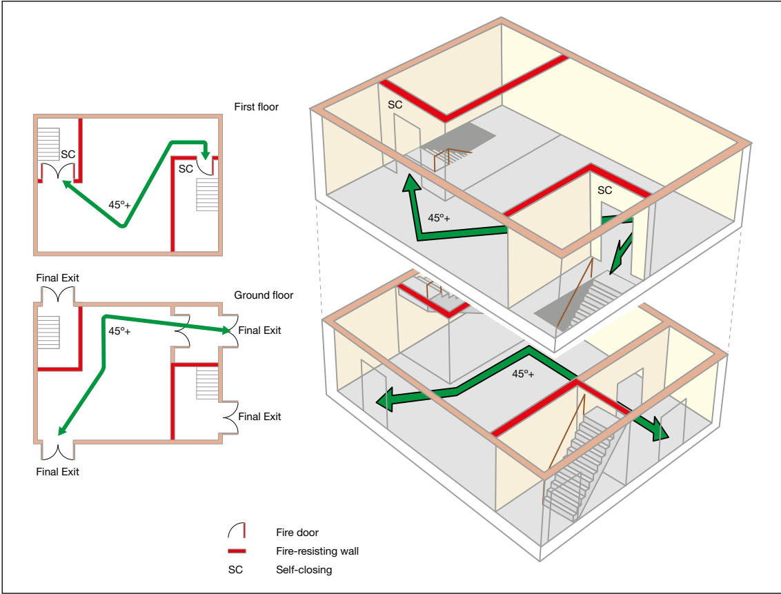
Figure 46: Two-storey premises: higher risk premises (e.g. nightclub)
