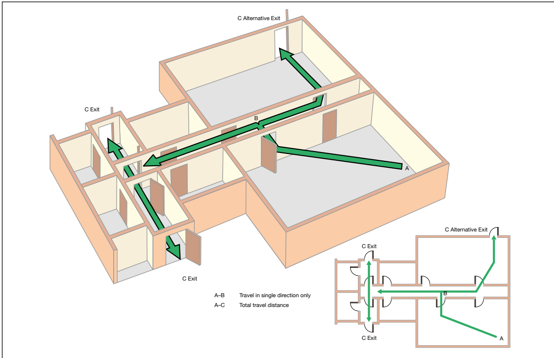
Figure 32: Dead-end condition provided with an alternative exit
