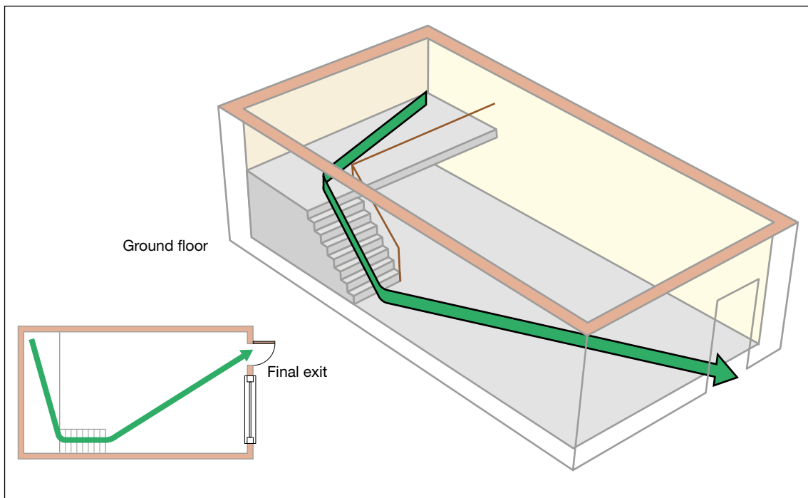
Figure 44: Ground floor premises with a single exit (including a mezzanine) (as part of larger premises)
