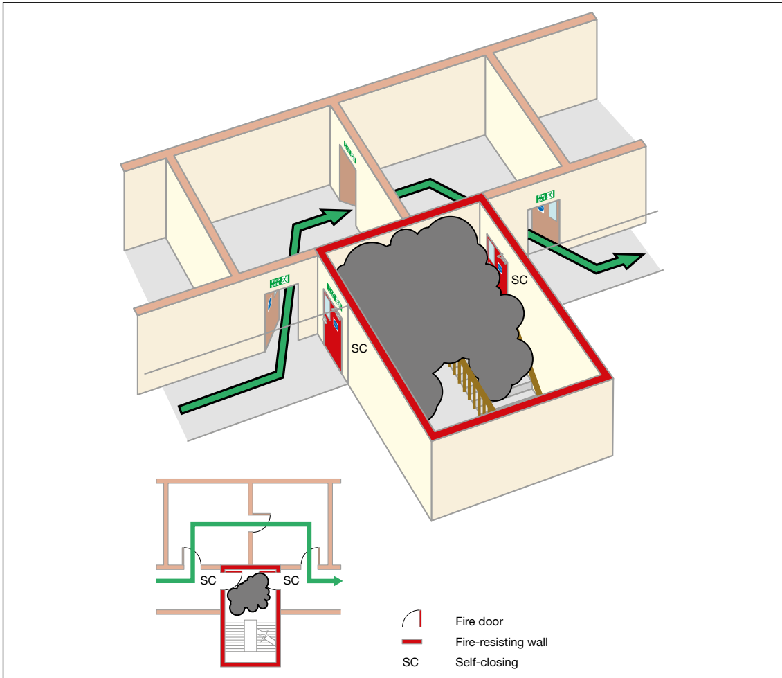
Figure 39: A stairway bypass route
