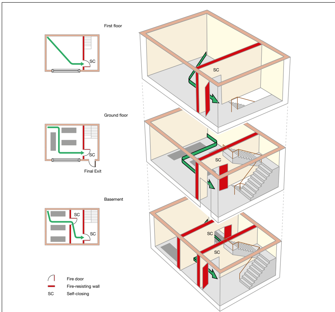
Figure 53: Three-storey premises, basement, ground and one upper floor
