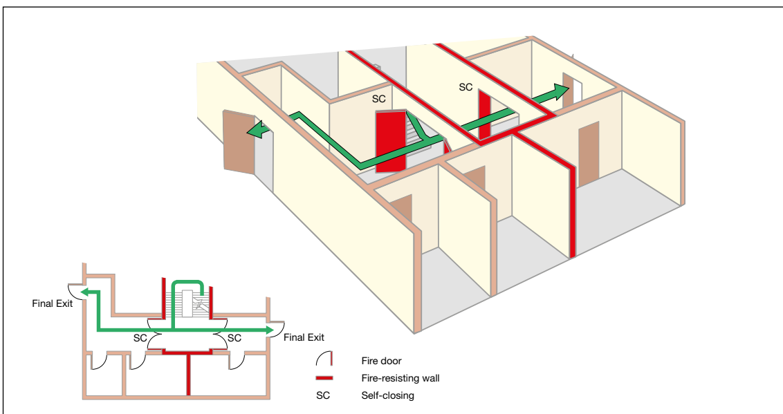
Figure 37: Example of two escape routes from a stairway to a final exits
