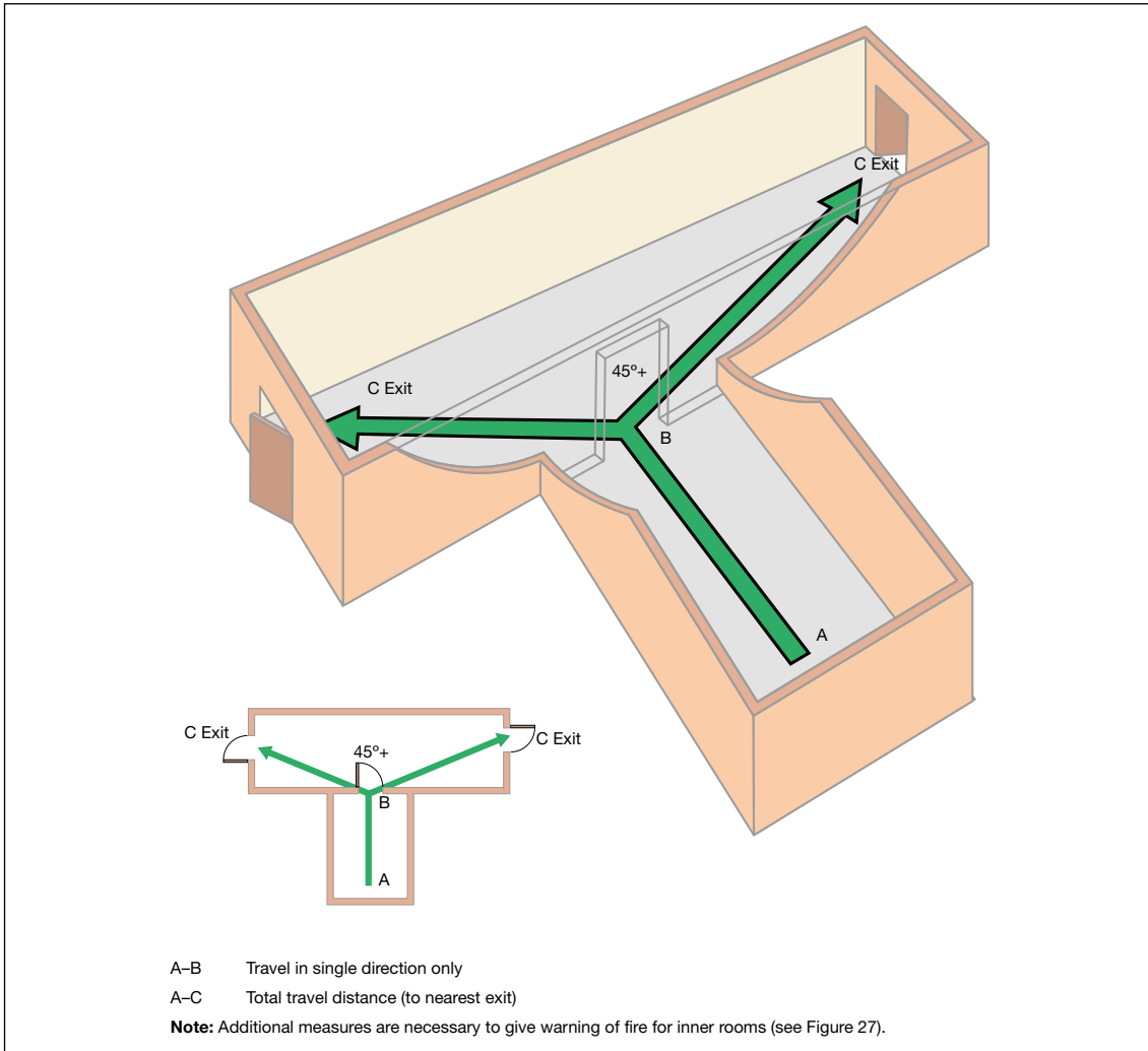
Figure 29: Measuring travel distance from initial dead end (inner room)
