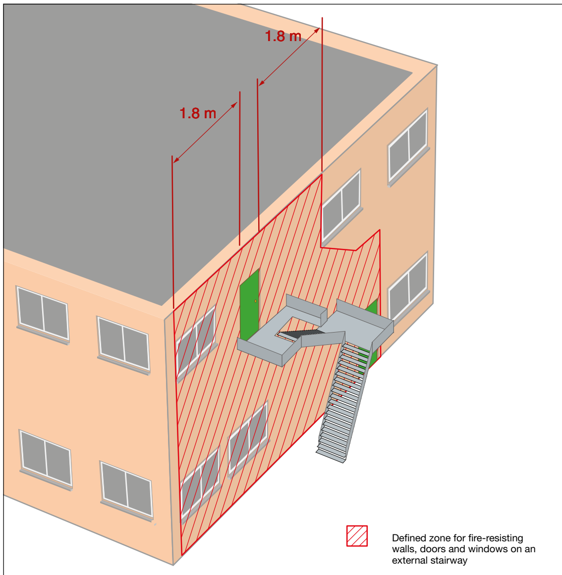
Figure 40: Protection to an external stairway
