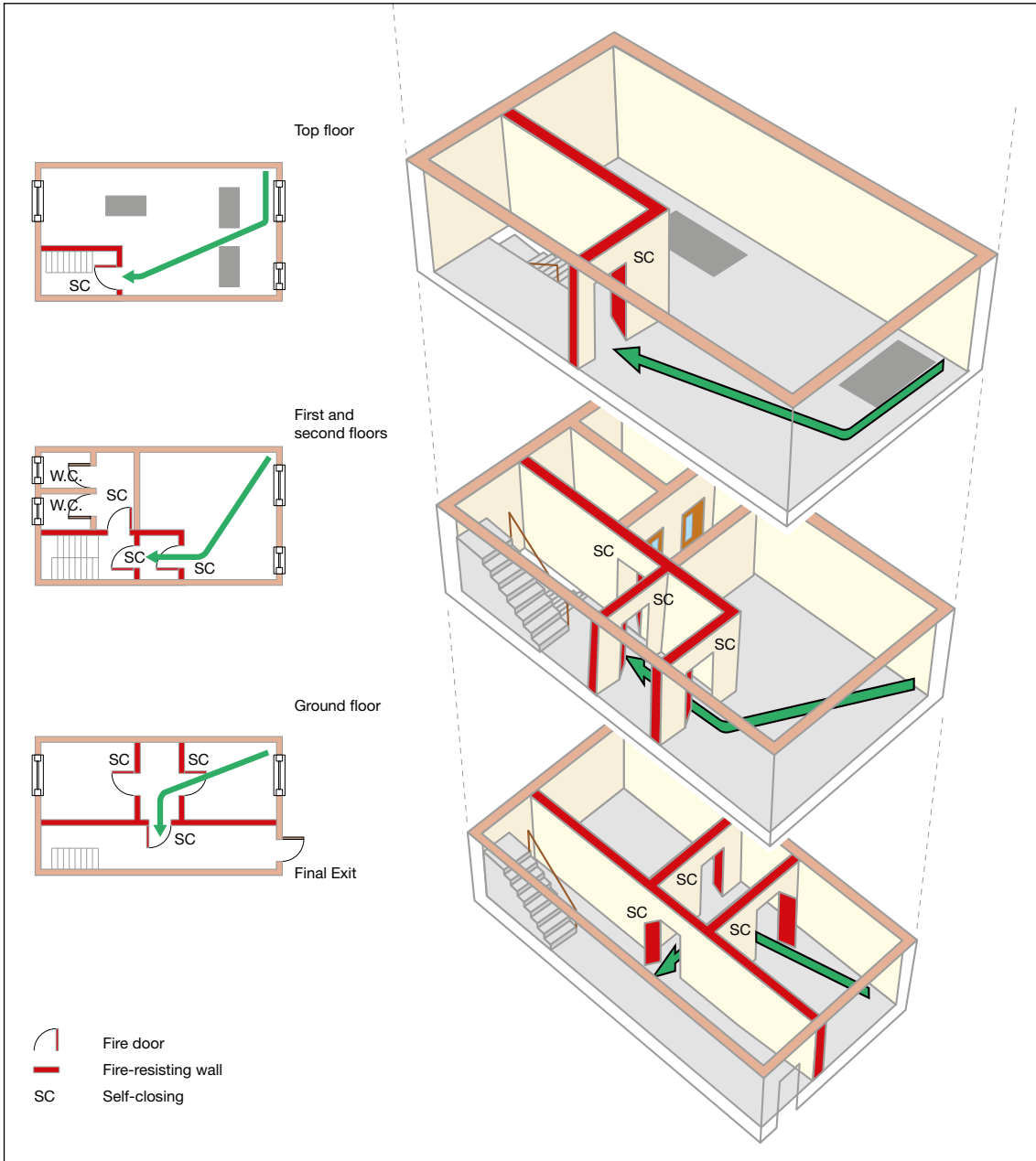
Figure 54: Four-storey, ground and up to three upper floors – protected by lobbies/corridors
