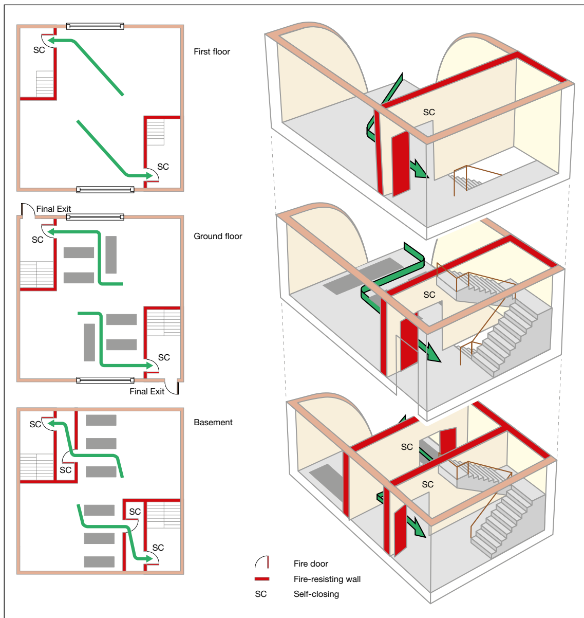
Figure 48: Four-storey premises, ground and up to three upper floors
