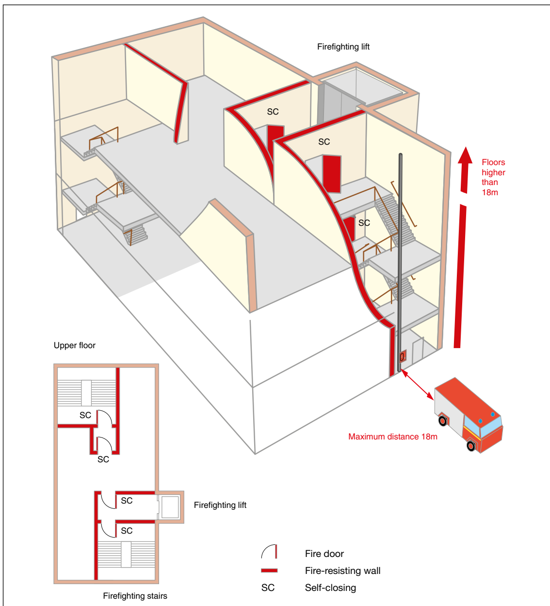
Figure 49: Tall building with a firefighting shaft
