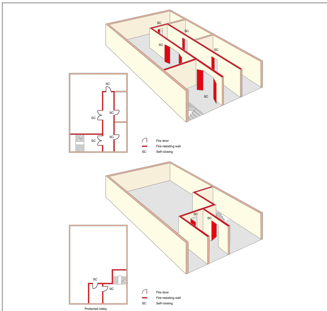
Figure 35: Examples of a stairway with protected lobby/corridor approach
