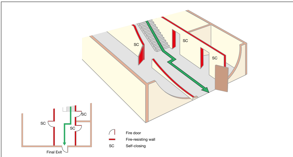
Figure 36: Example of a protected route from a stairway to a final exit
