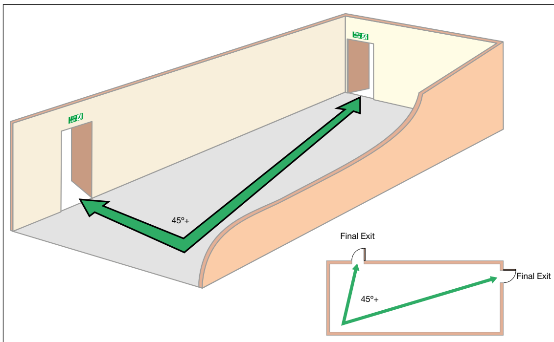
Figure 42: Ground floor premises with more than one exit
