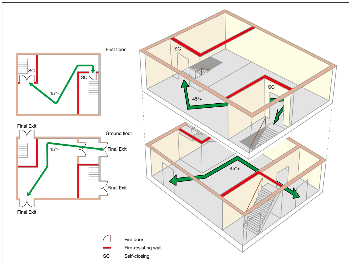
Figure 45: Two-storey premises: lower risk premises (e.g. church hall)
