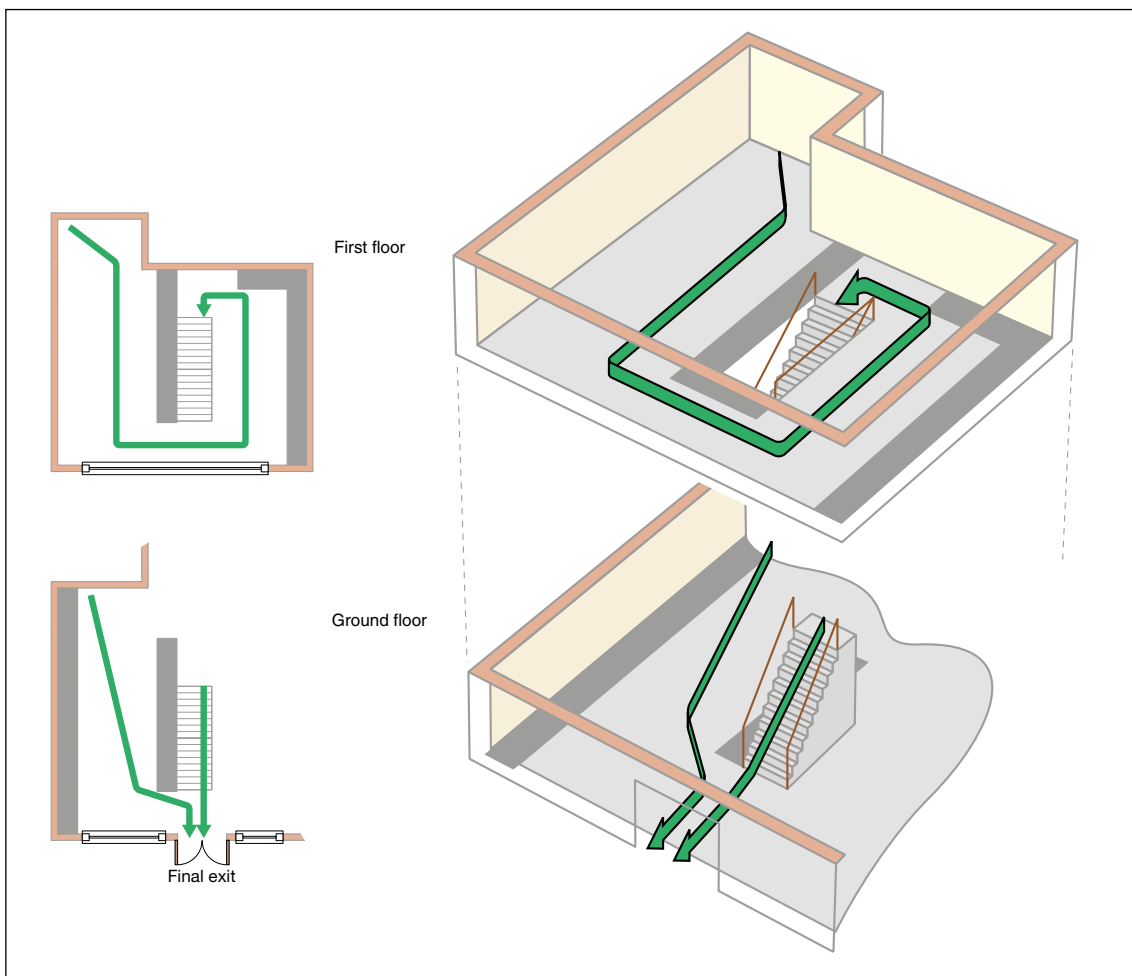
Figure 50: Two-storey premises, ground and one upper floor
