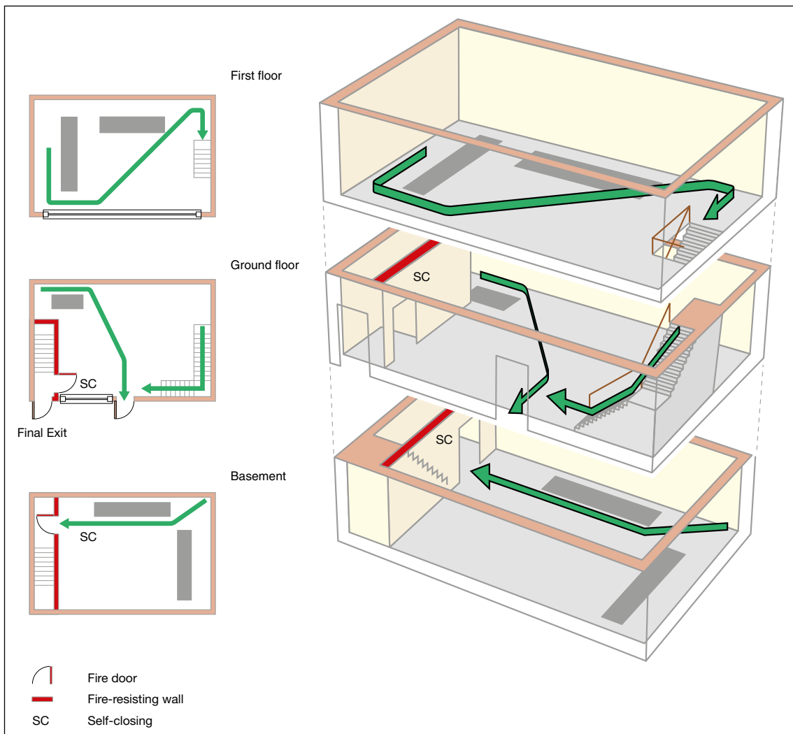
Figure 51: Three-storey, small basement, ground and one upper floor, with a separate single stairway to each
