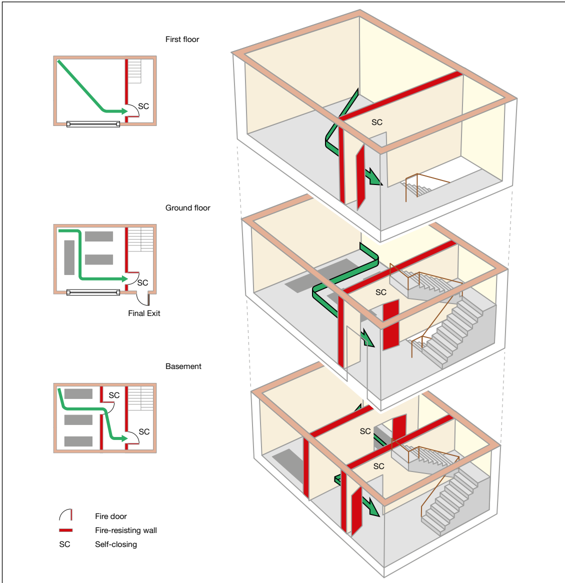
Figure 52: Three-storey, basement, ground and one upper floor, with a single stairway
