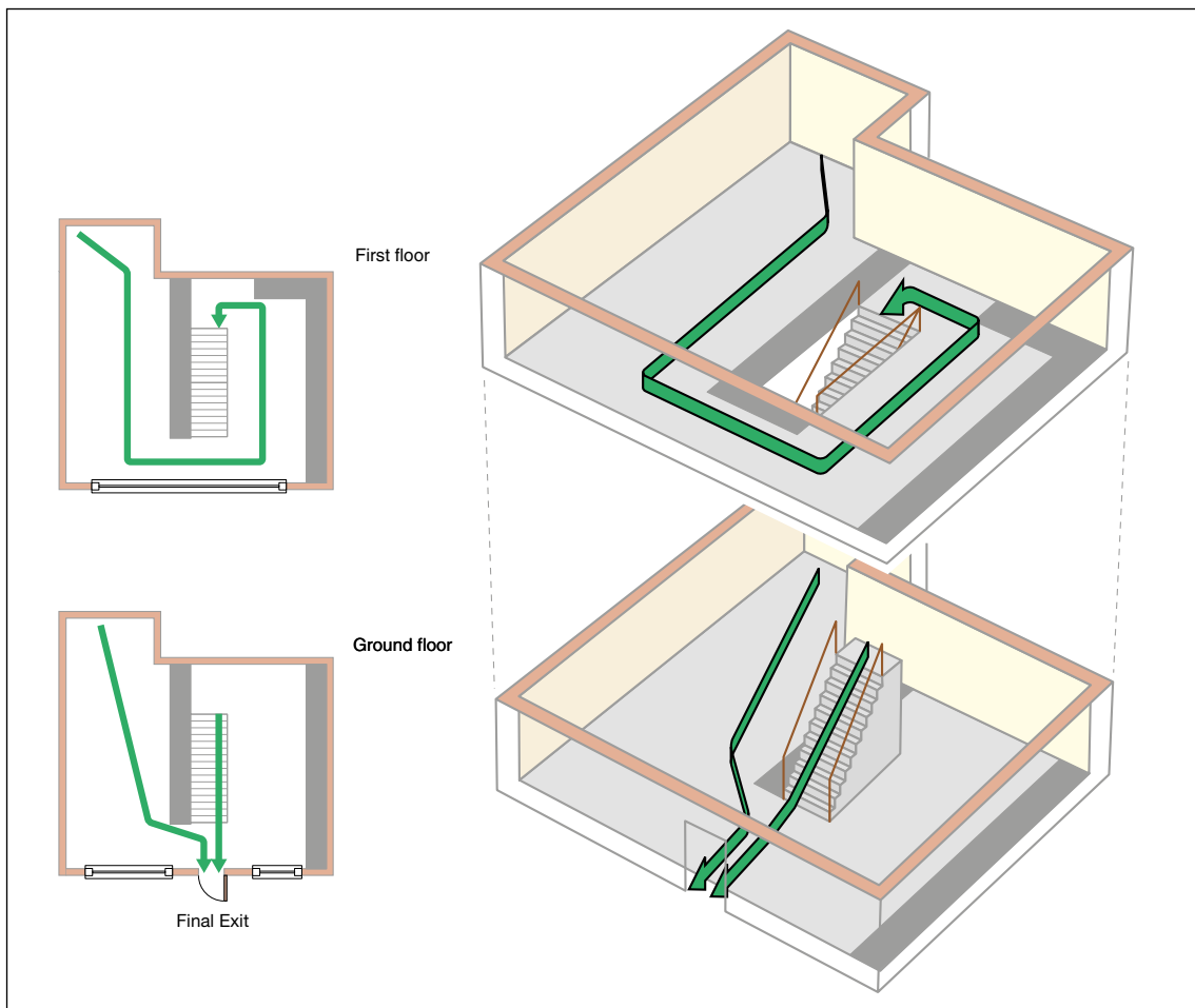
Figure 49: Two-storey, ground and one upper floor with a single stairway
