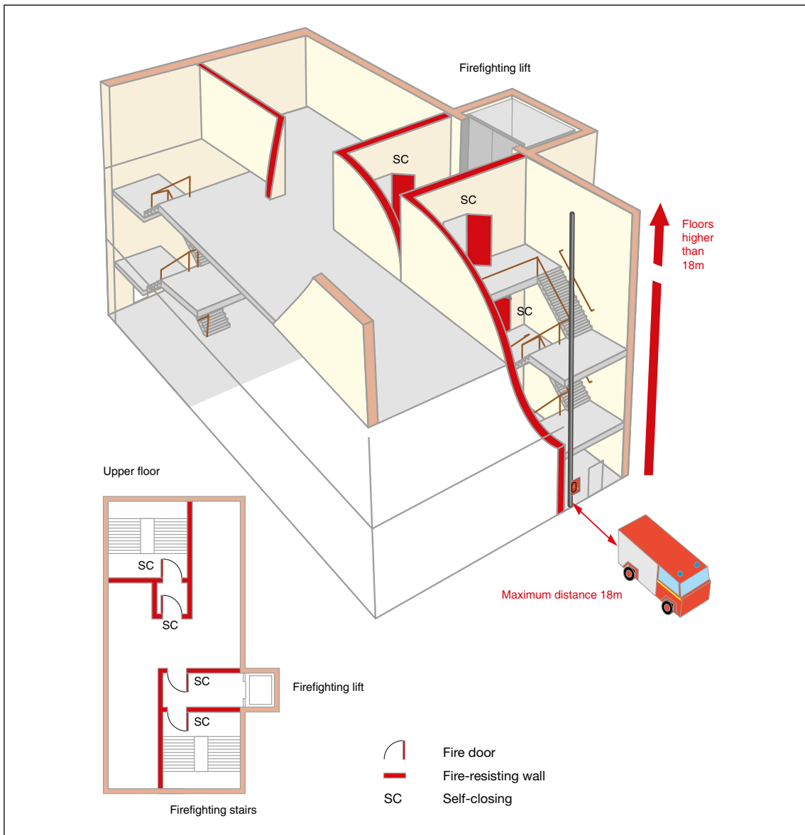
Figure 48: Tall building with a firefighting shaft
