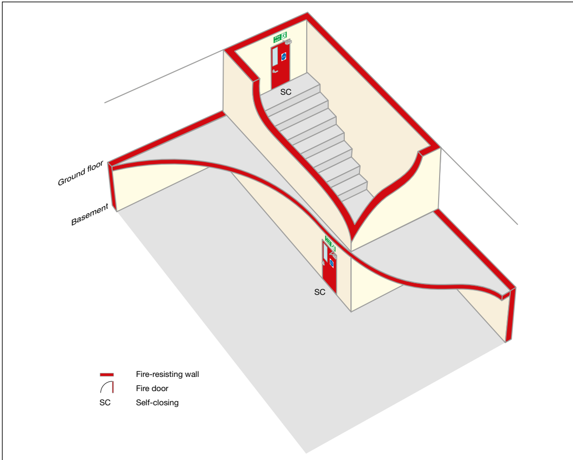
Figure 32: Basement protection
