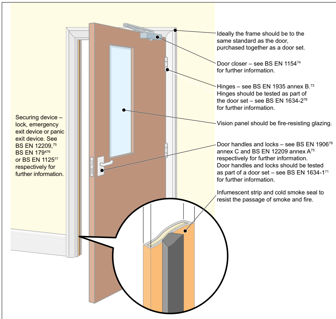
Figure 66: A fire-resisting and smoke-stopping door
