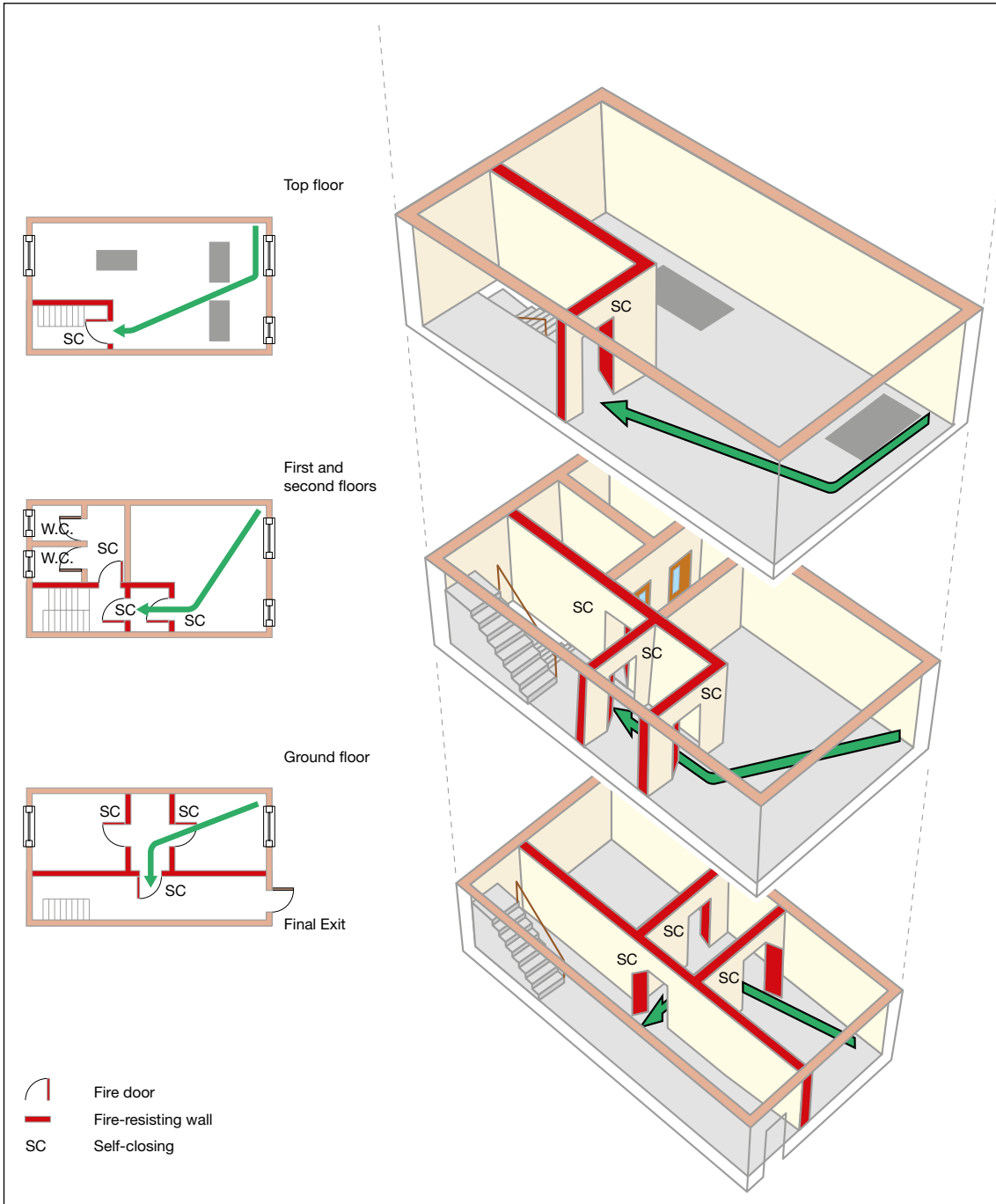
Figure 54: Four storey, ground and up to three upper floors: higher risk premises – protected lobbies/corridors
