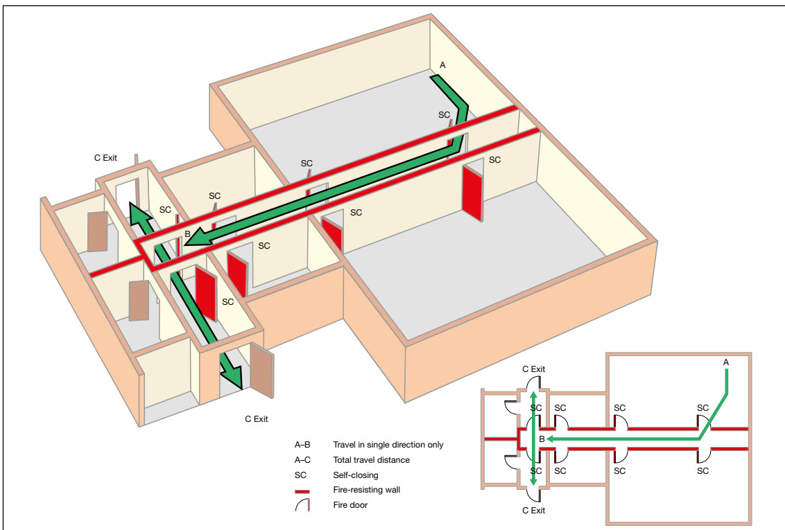
Figure 30: Dead-end conditions with fire-resisting construction
