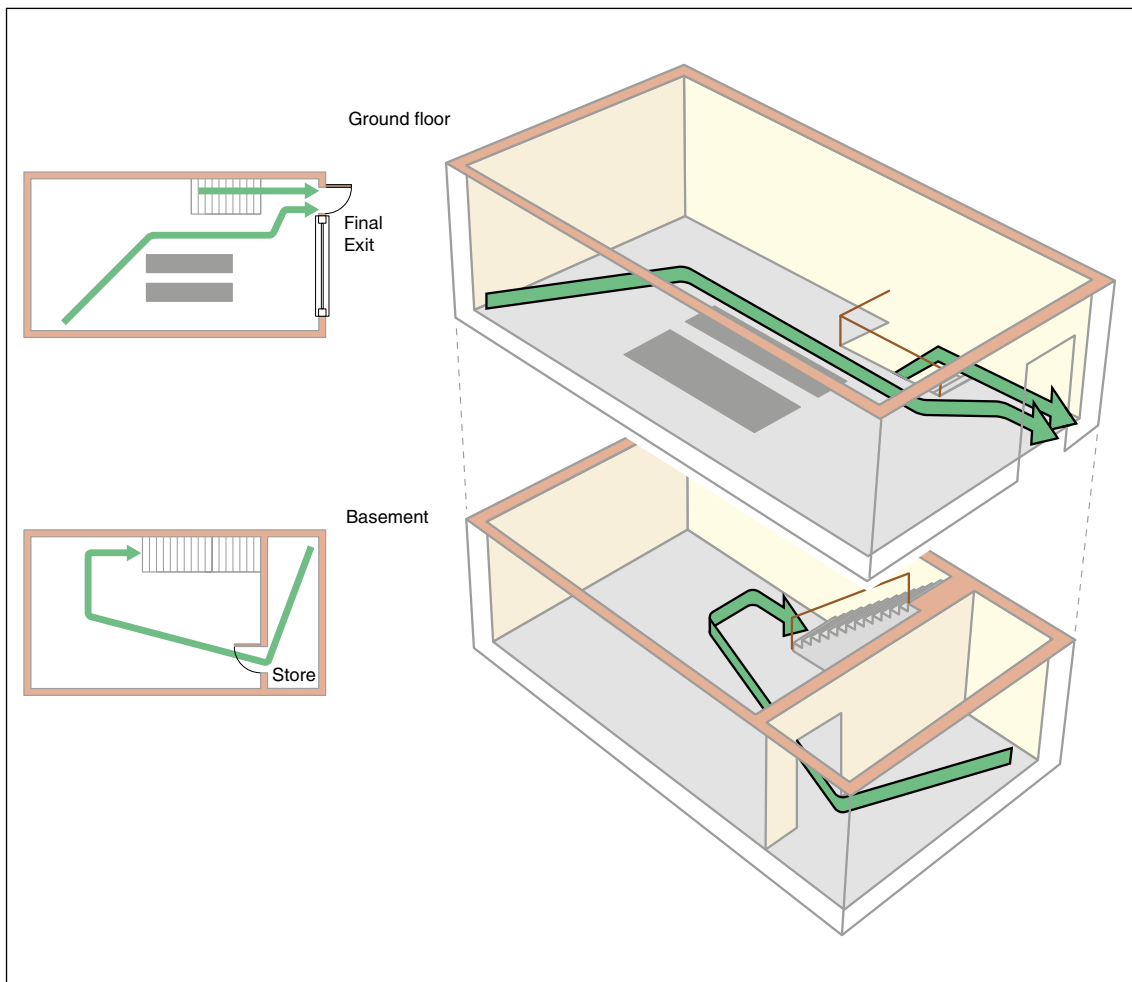
Figure 50: Two-storey, with a single stairway, basement and ground floor
