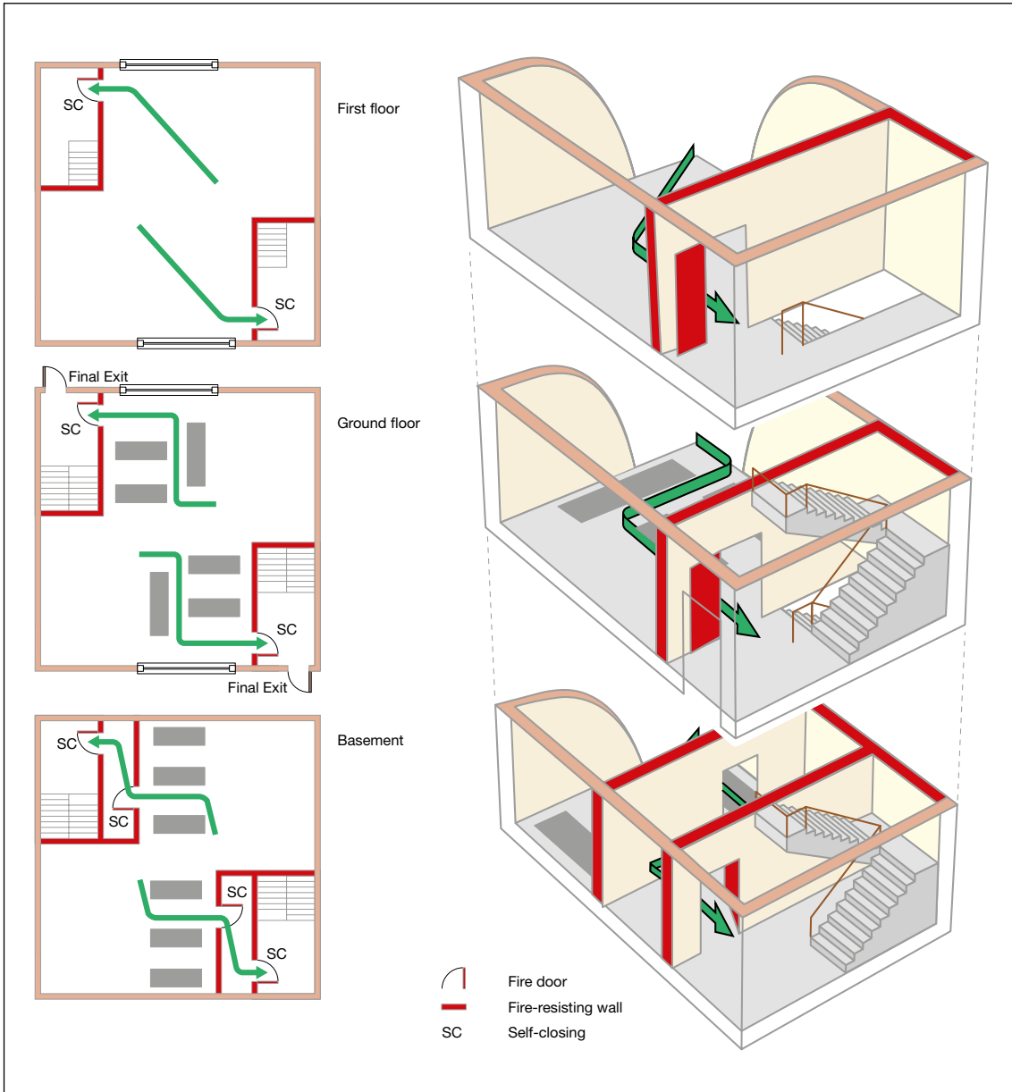
Figure 46: Three-storey, basement, ground and one upper floor
