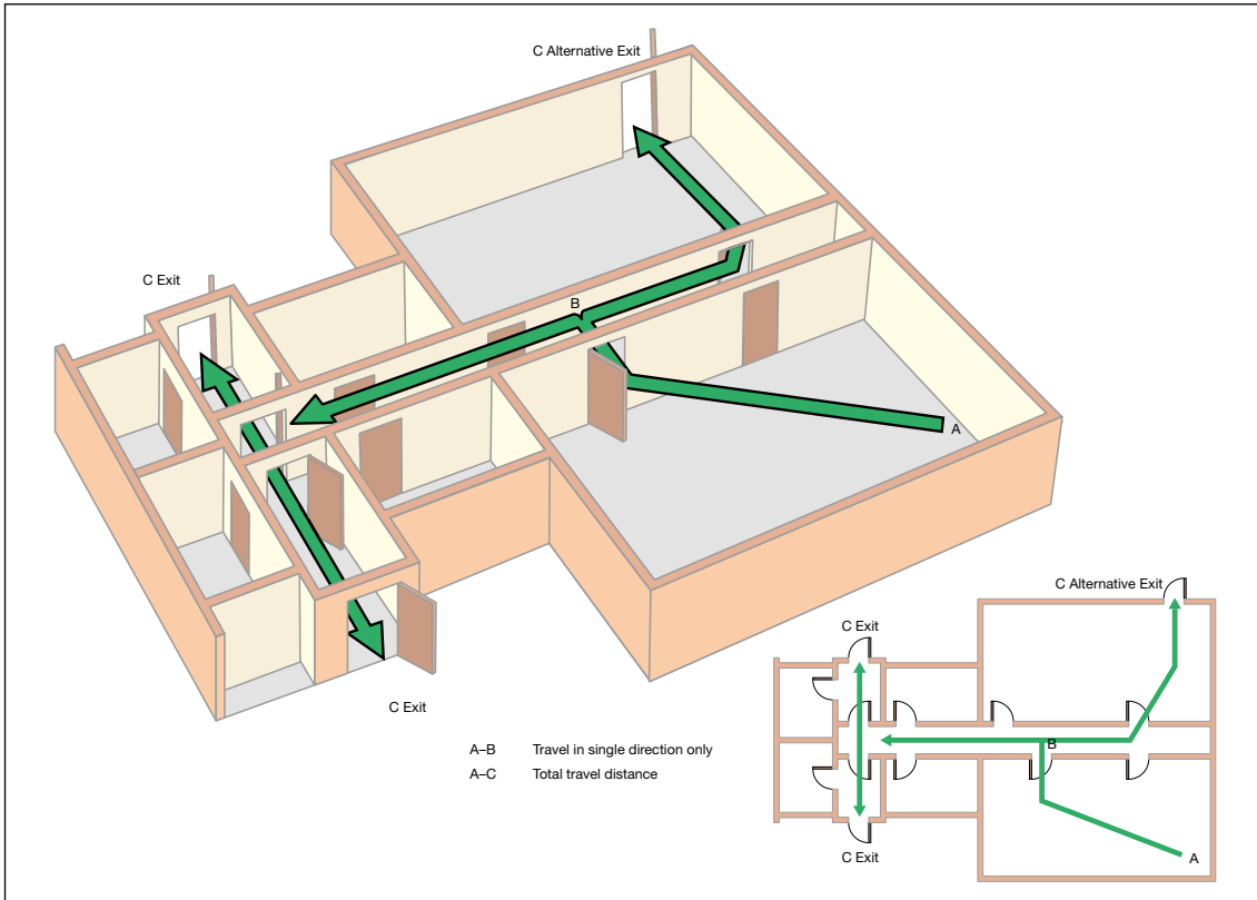
Figure 31: Dead-end conditions provided with an alternative exit
