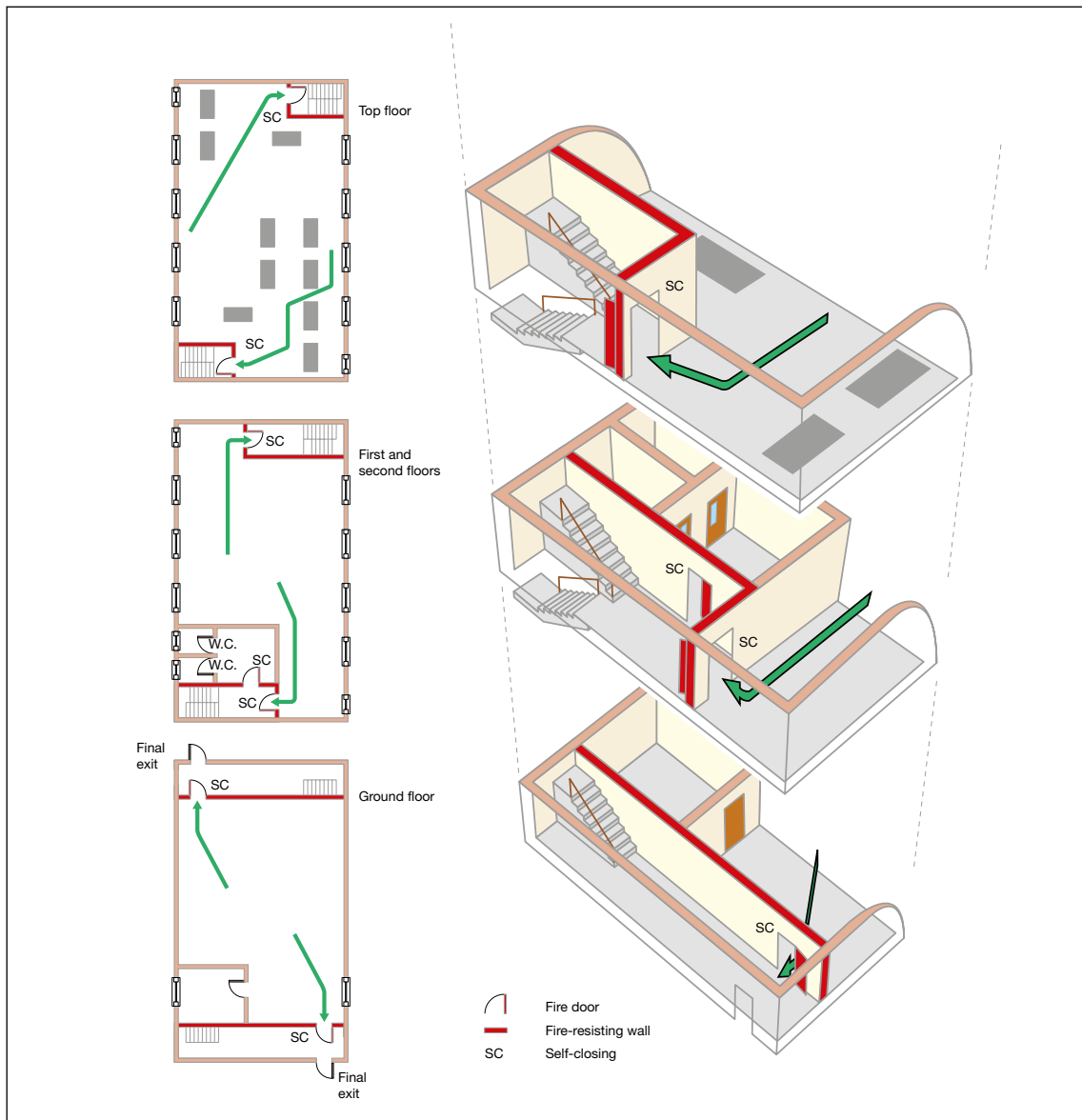
Figure 47: Four-storey, ground and up to three upper floors
