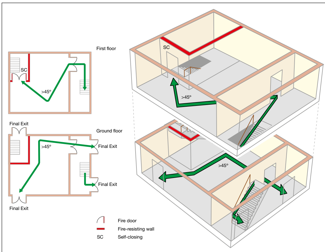
Figure 44: Two-storey, ground and one upper floor: lower risk premises (e.g. a warehouse storing sand, gravel and cement)
