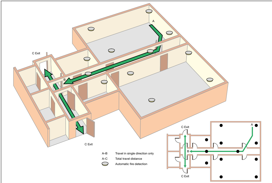
Figure 29: Dead-end conditions with automatic fire detection
