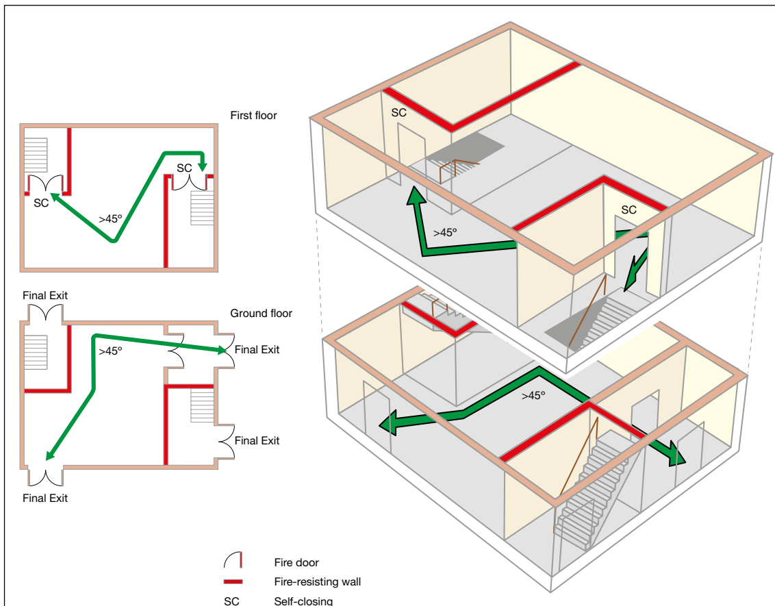
Figure 45: Two-storey, ground and one upper floor: higher risk premises (e.g. a factory with paint spraying activities)
