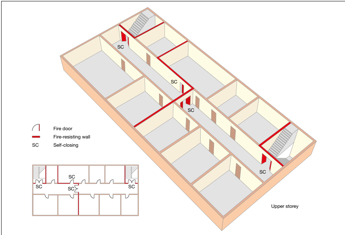
Figure 33: Subdivision of corridor between two stairways or exits
