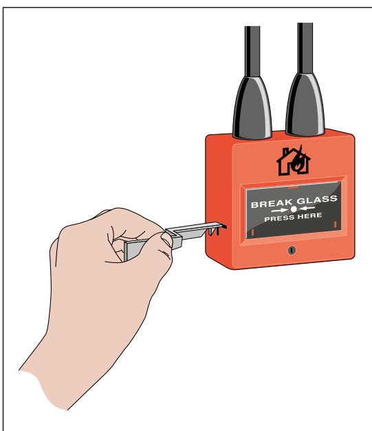
Figure 18: Using a test key
