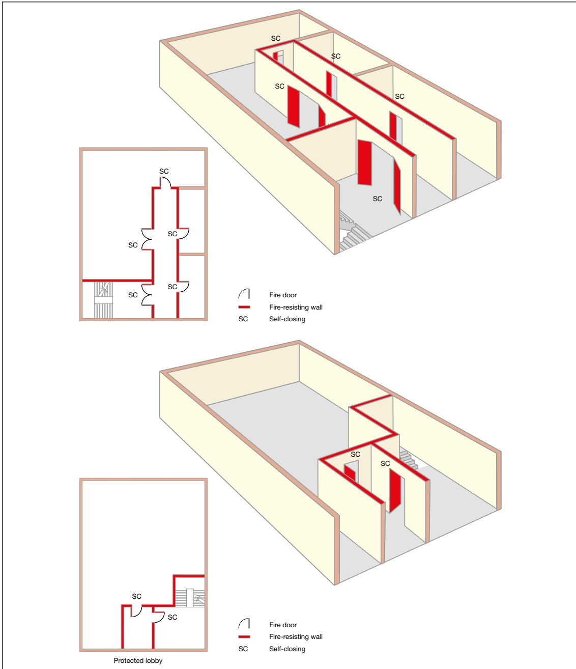
Figure 34: Examples of a stairway with protected lobby/corridor approach
