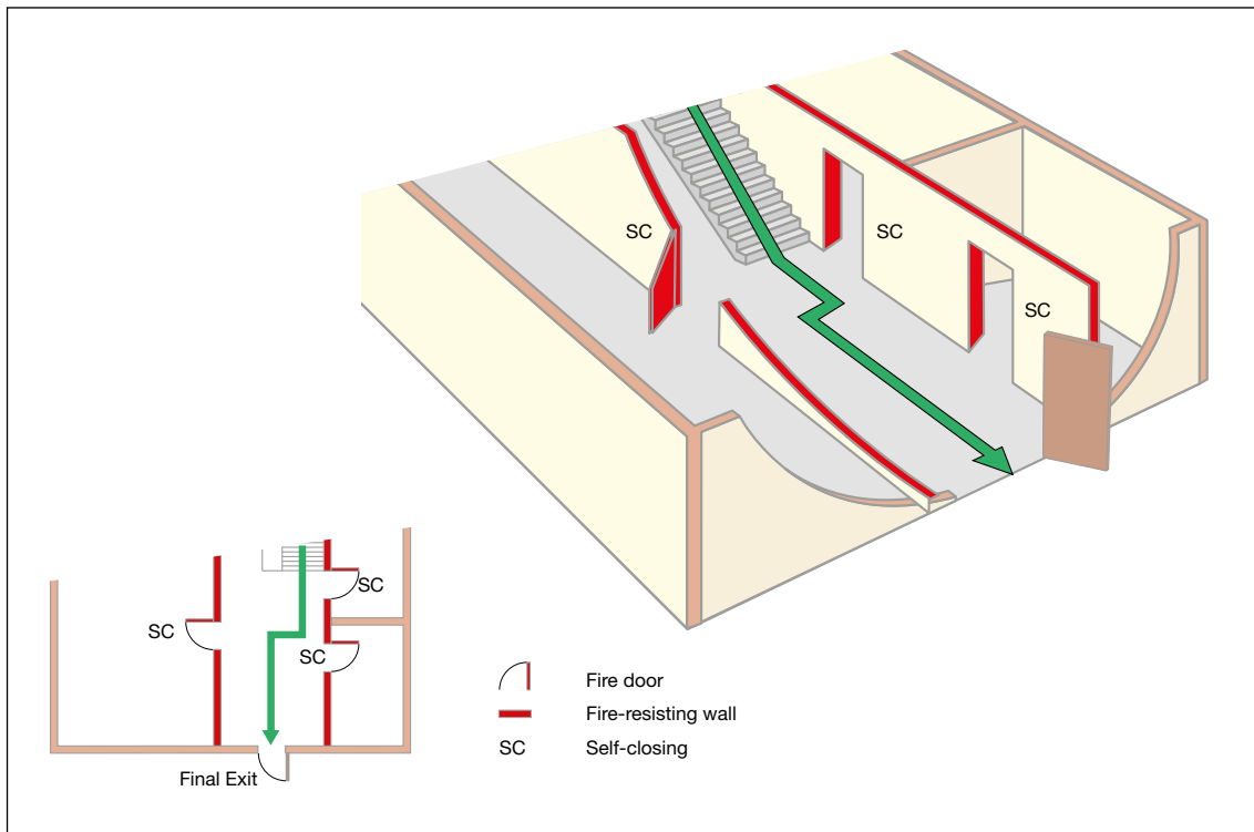
Figure 35: Examples of a protected route from a stairway to a final exit
