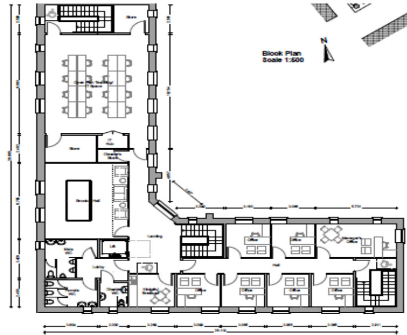
Proposed First Floor Spatial Plan Scale 1:100
