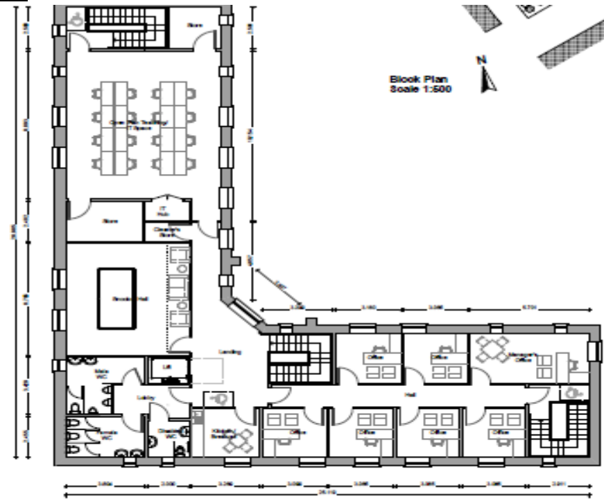
Proposed First Floor Spatial Plan Scale 1:100
