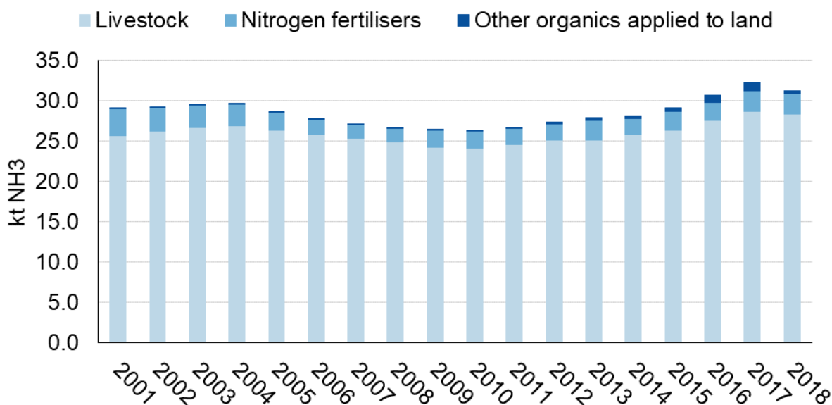
Figure 3.3 Annual ammonia emissions from agriculture, 2001 – 2018
