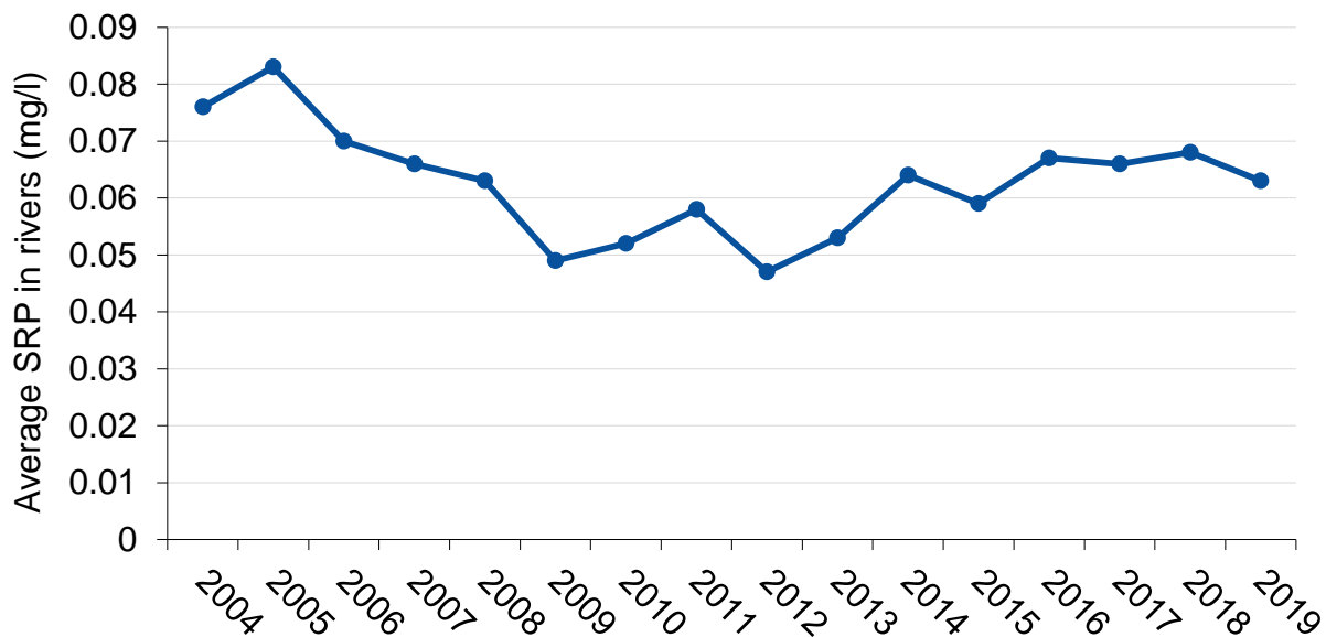
Figure 4.3 soluble reactive phosphorus (SRP) in rivers, 2004 – 2019
