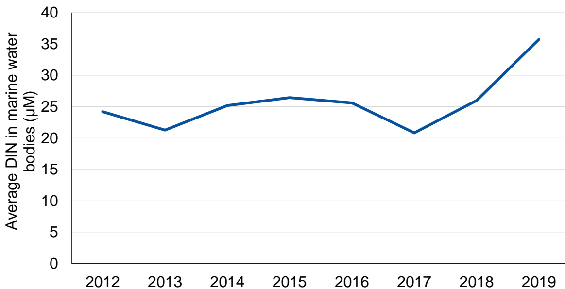
Figure 4.4 Winter Dissolved Inorganic Nitrogen (Winter DIN), 2012 - 2019
