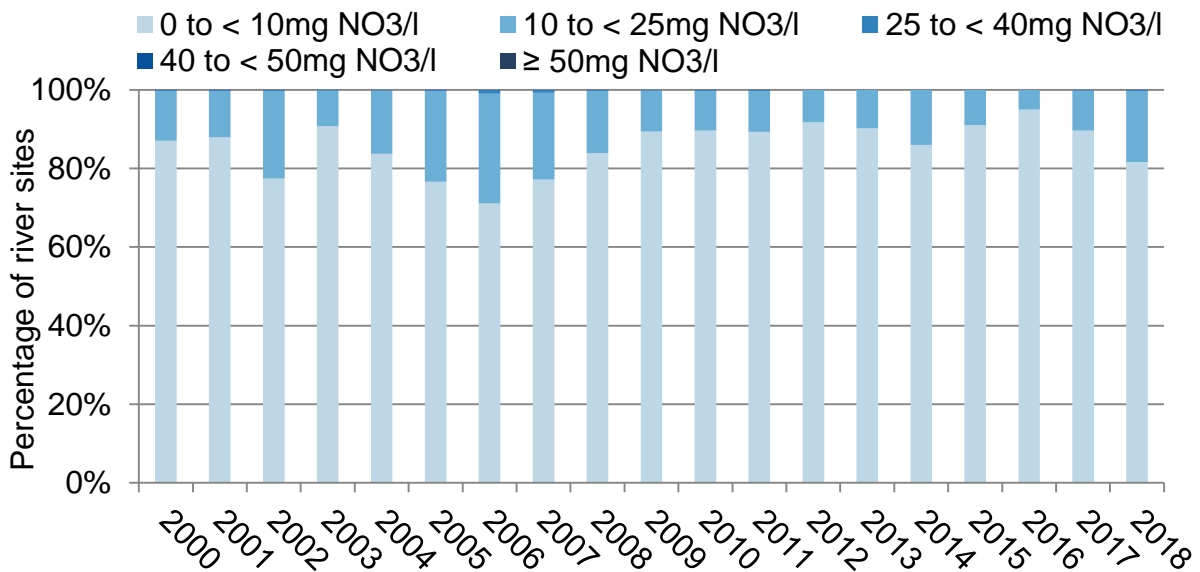
Figure 4.2 Annual mean nitrate concentrations (in rivers), 2000 – 2018
