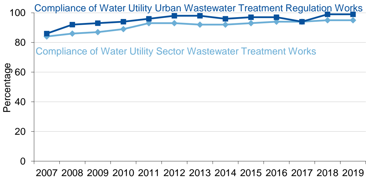
Figure 4.6 Summary of compliance of Water Utility Waste Water Treatment Works (WWTW), 2007 – 2019
