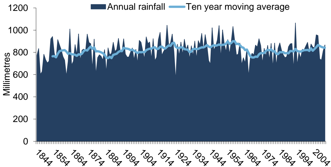
Figure 2.4 Annual rainfall, 1853 – 2019
