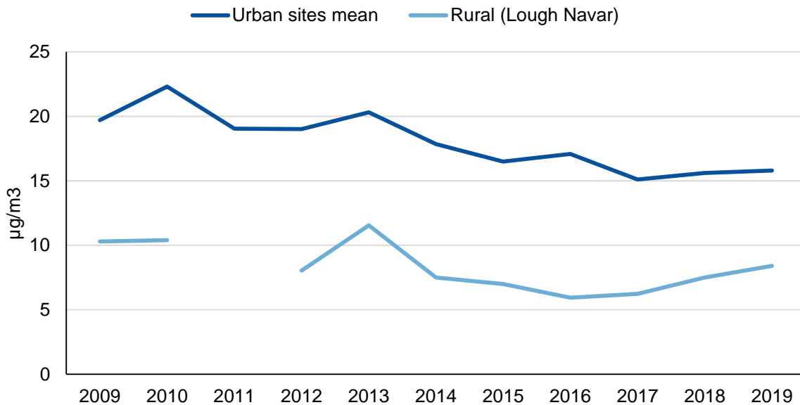
Figure 3.2 Annual mean concentration of particulate matter (PM 10 ), 2009 – 2019
