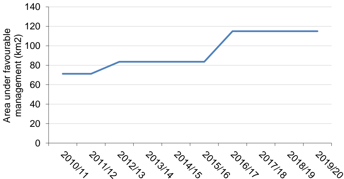
Figure 5.4 Marine protected sites under favourable management 2010/11 to 2019/20
