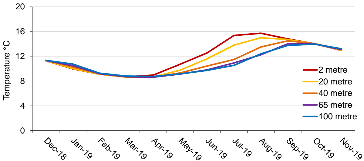
Figure 4.9 Average monthly sea temperature by depth, Irish Sea, Dec18 – Nov19
