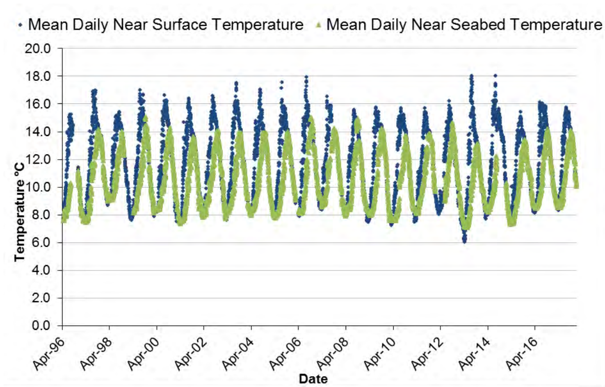
Figure 4.6 Daily sea temperature, Irish Sea, April 1996 - December 2017
