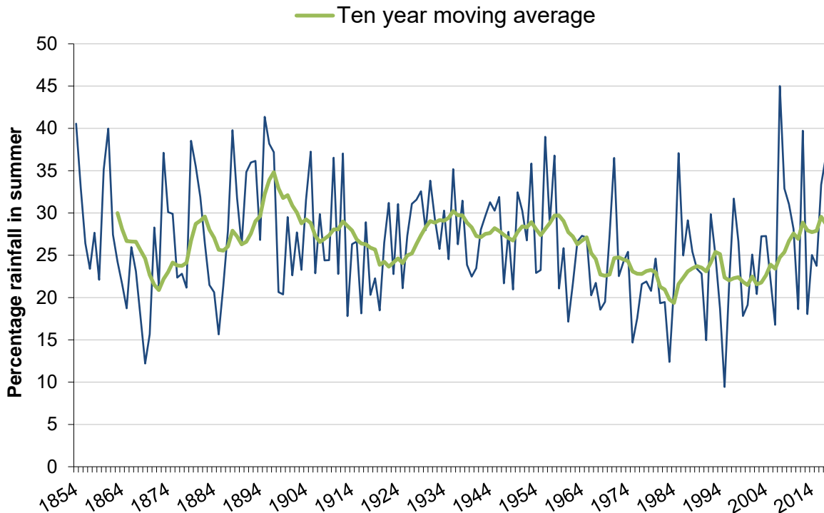
Figure 2.15 Percentage of annual rainfall falling in summer (Jun – Aug), 1854 – 2017
