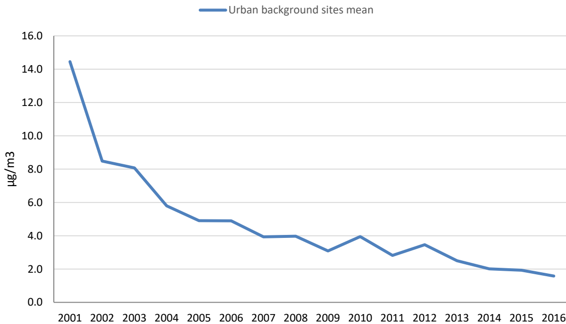
Figure 2.5 Annual mean concentration of sulphur dioxide (SO 2 ), 2001 – 2016
