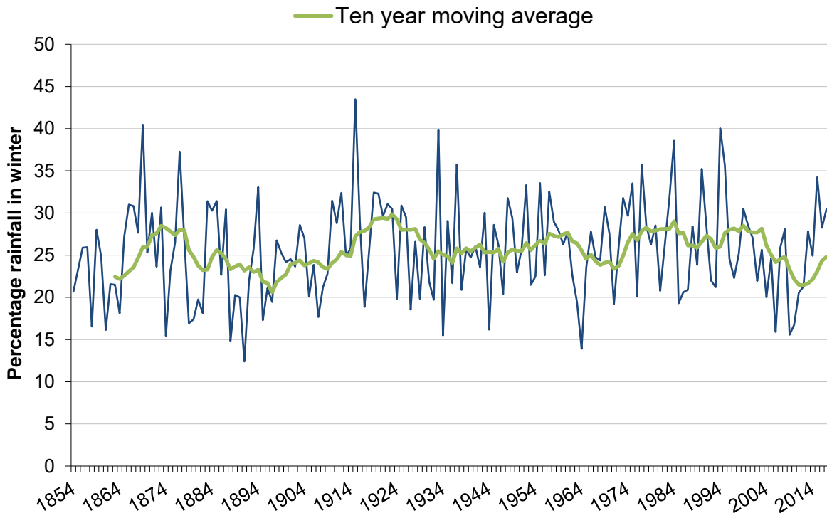
Figure 2.14 Percentage of annual rainfall falling in winter (Dec – Feb), 1854 – 2017
