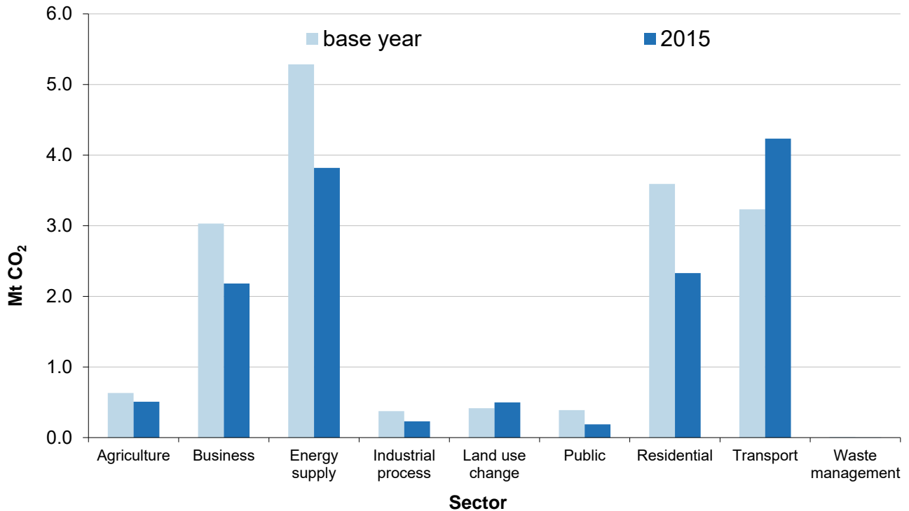
Figure 2.9 Carbon dioxide (CO 2 ) emissions in Northern Ireland by sector, base year & 2015
