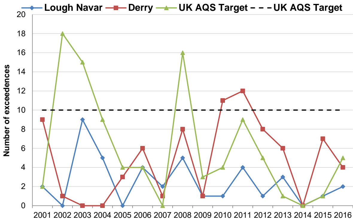
Figure 2.3 Annual exceedences of 8-hour mean objective for ozone, 2001 – 2016
