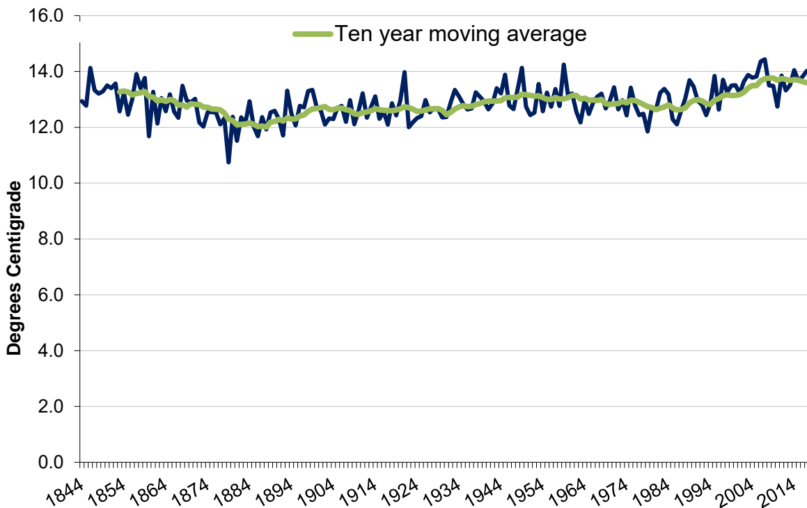
Figure 2.13 Mean annual maximum temperature, 1844 – 2017
