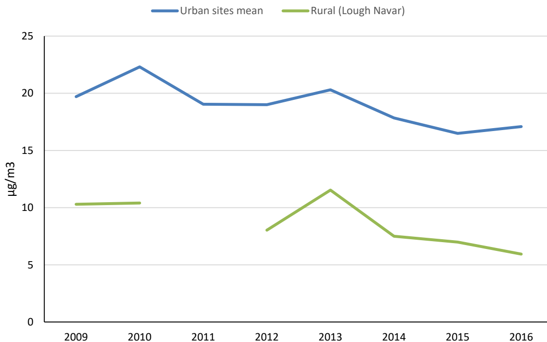
Figure 2.2 Annual mean concentration of particulate matter (PM 10 ), 2009 – 2016
