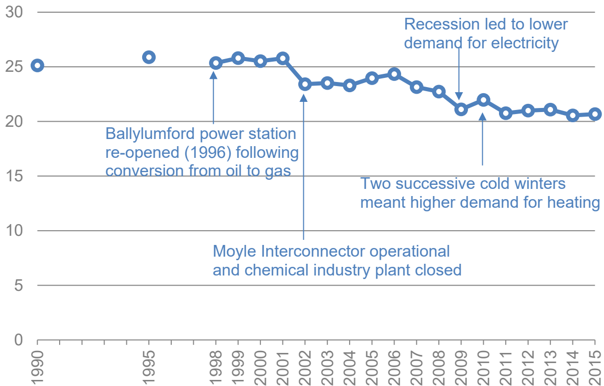
Figure 2.7 Total greenhouse gas emissions in Northern Ireland, 1990 – 2015
