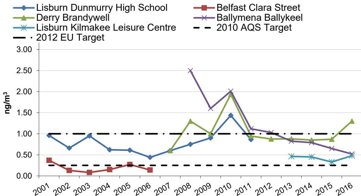
Figure 2.4 Annual mean concentrations of Benzo(a)pyrene, 2001 – 2016
