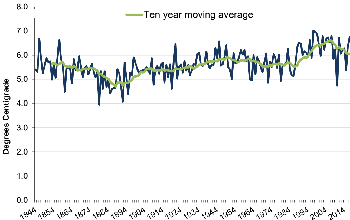
Figure 2.12 Mean annual minimum temperature, 1844 – 2017
