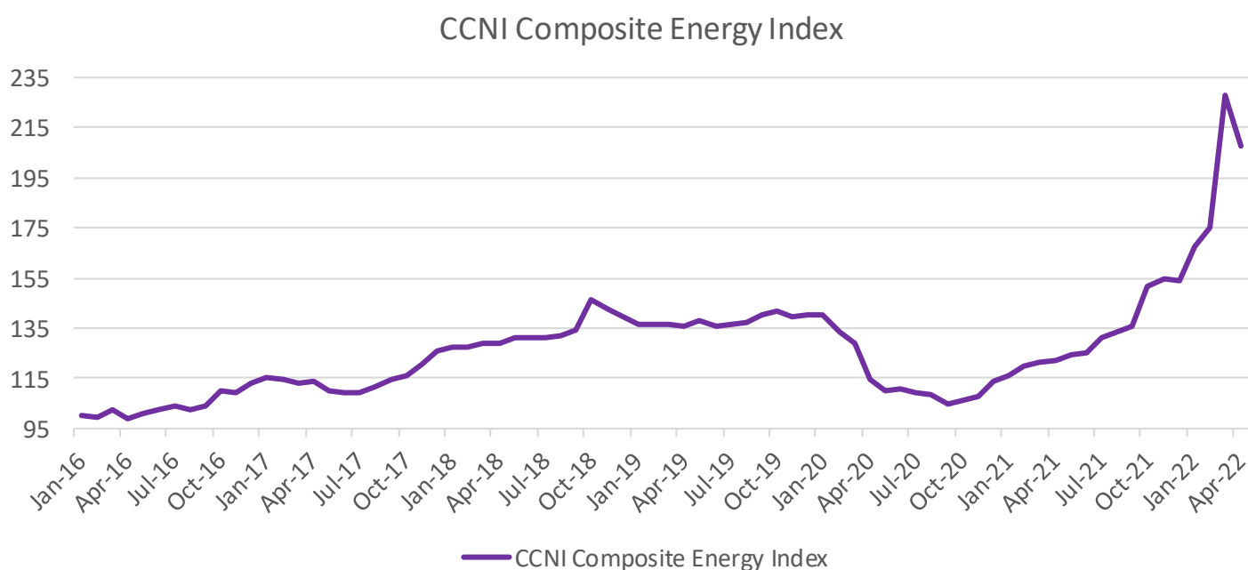
Figure 1: Home Energy Index (composite of electricity, gas and HHO) for Northern Ireland (January 2016 – April 2022).
