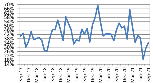
Figure 2: Monthly % of Electricity Consumption from Renewable Sources (Sept 2017 – Sept 2021)
