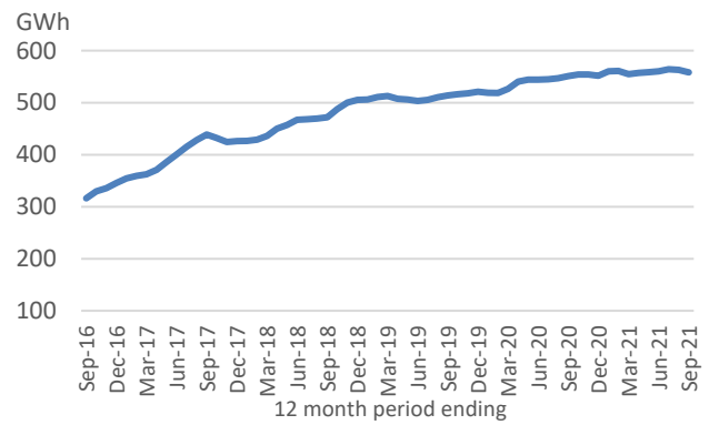
Figure 6: Rolling 12 month Volume of Non-wind Renewable Electricity Generation (September 2016 – September 2021)
