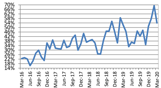
Figure 2: Monthly % of Electricity Consumption from Renewable Sources (Mar 2016 – Mar 2020)
