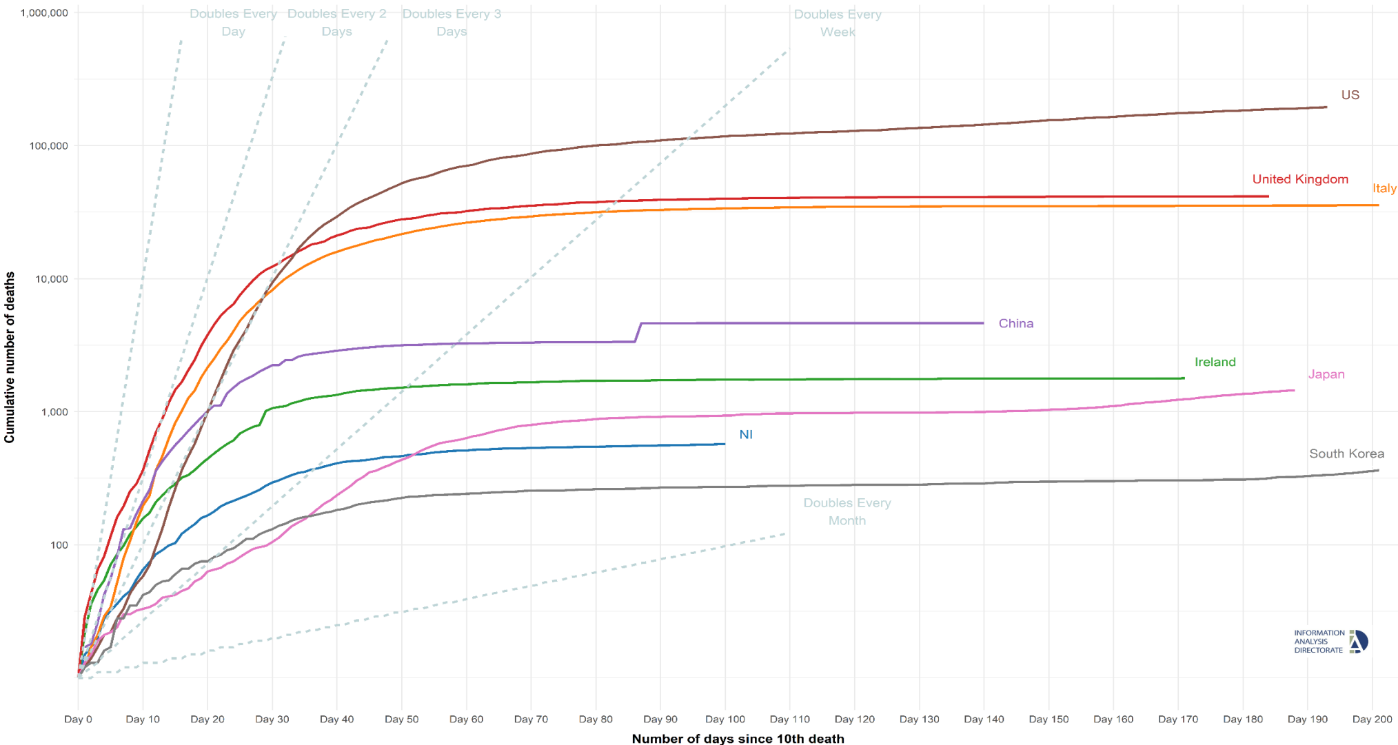
Figure 2: Cumulative number of deaths after the 10th death, where the deceased has had a positive test for COVID-19 and died within 28 days, whether or not COVID-19 was the cause of death. The 10th death for all countries are aligned by calculating the first time the number of deaths was greater than or equal to 10 and rounding down to exactly 10.
