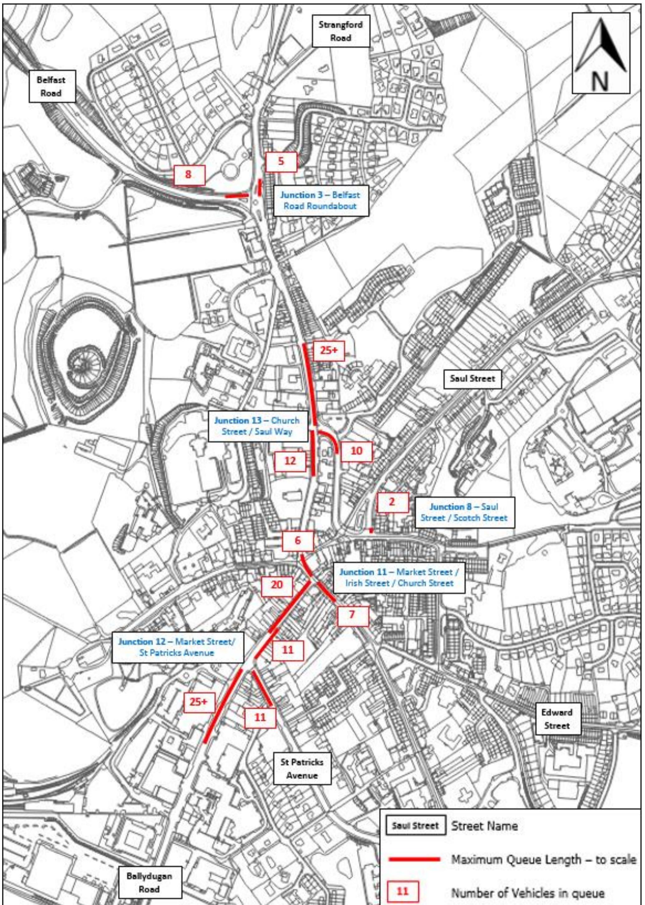
Queue Figure 2: Maximum Queue Length PM (North-western sites)
