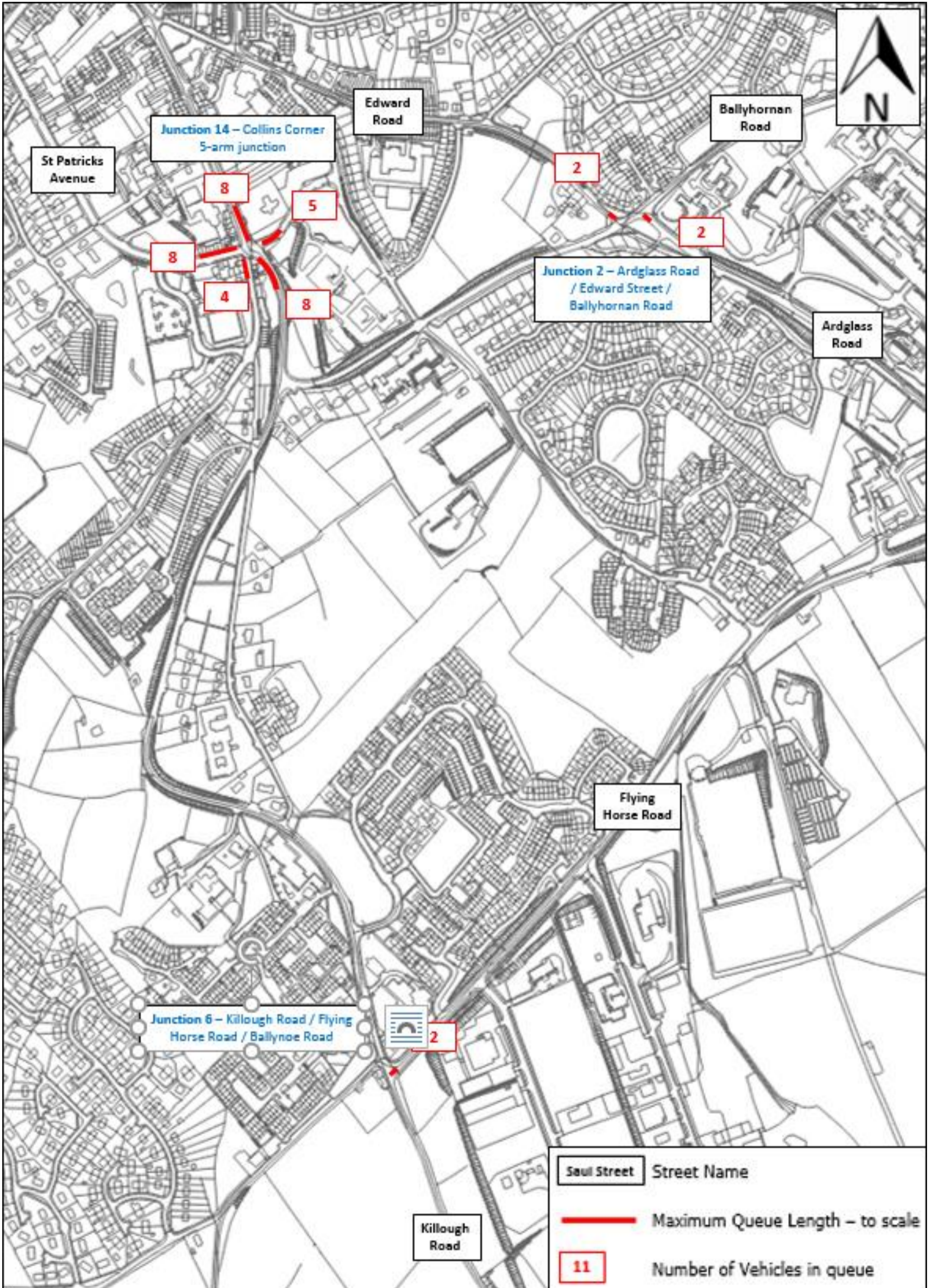
Queue Figure 4: Maximum Queue Length PM (South-eastern site)
